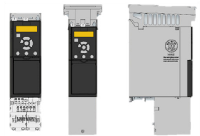
Illustration 26: Drive with Conversion Kit Components
