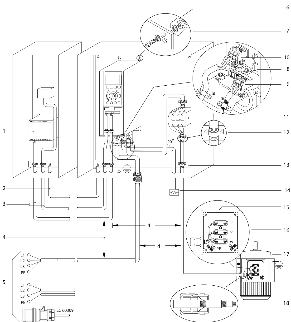
Illustration 28: Typical Electrical Connection
