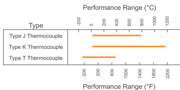
Figure 4: Thermocouple Temperature Ranges
