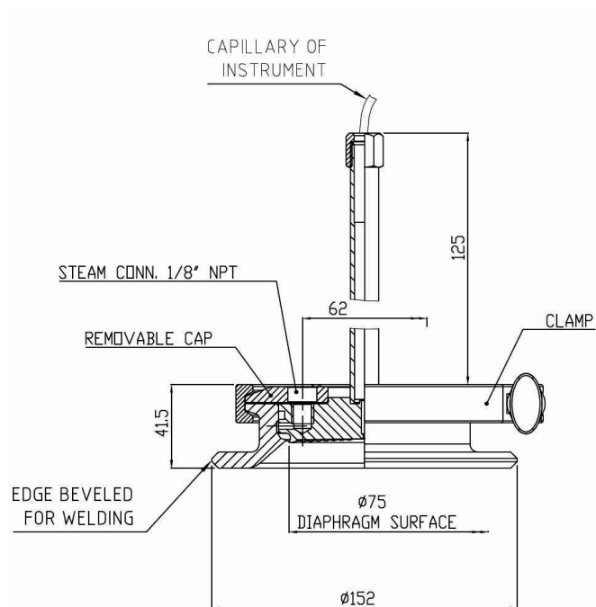
Figure 30: Sanitary spud and welding point
