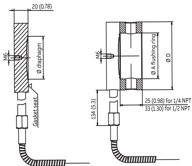
ASME and EN 1092-1 Form B1 smooth and serrated
