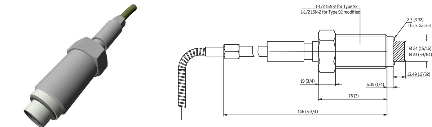
Figure 12: 1-1/2 in. threaded union type 92 or 92 modified
