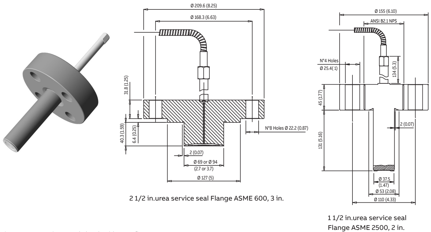
Figure 9: Urea service extended seals with ASME flange
