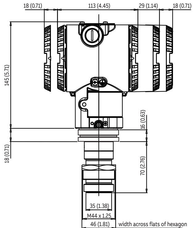
Figure 28: S26KN with M44 x 1.5 threaded spud connection
