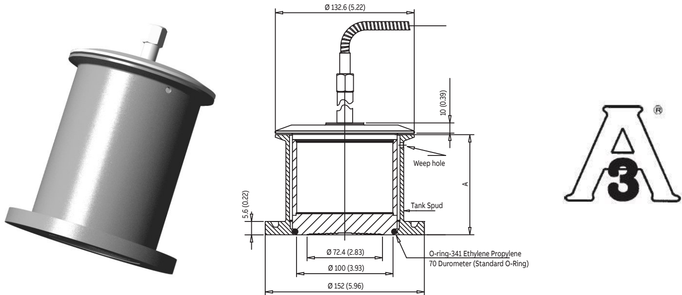
Figure 18: Sanitary seal with extended diaphragm
