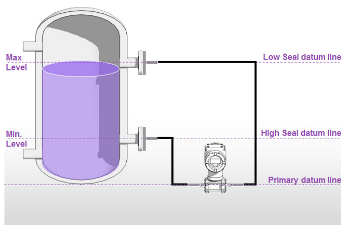
Figure 34: Level measurement of a liquid in a closed tank - vacuum or pressure service
