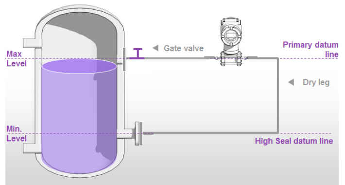
Figure 40: Level measurement of a liquid in a closed tank - vacuum or pressure service - dry leg installation
