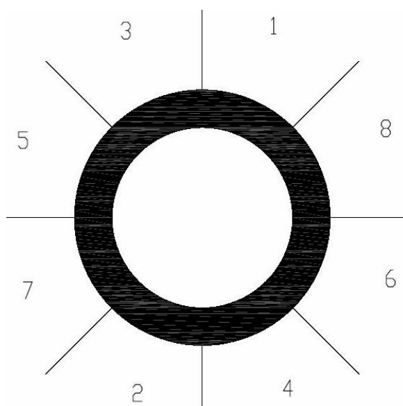
Figure 29: Welding sequence for spuds
