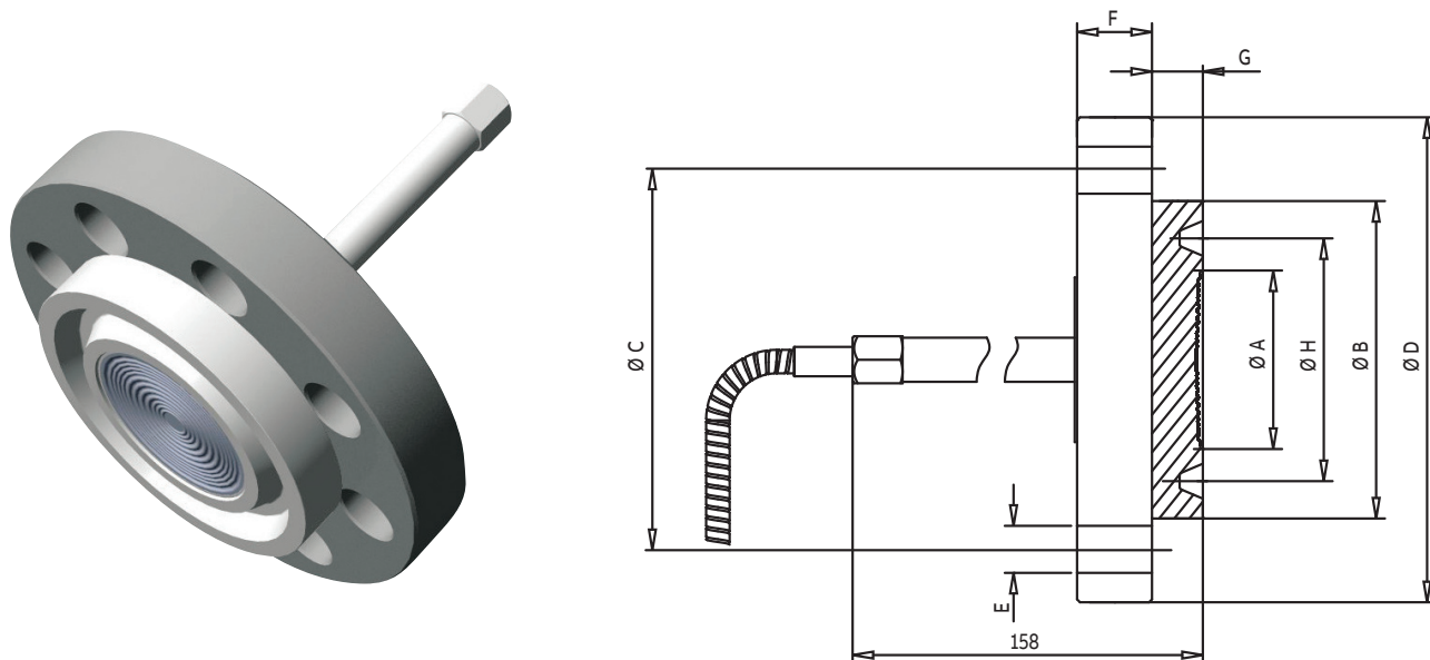
Figure 5: Ring-joint diaphragm seal
