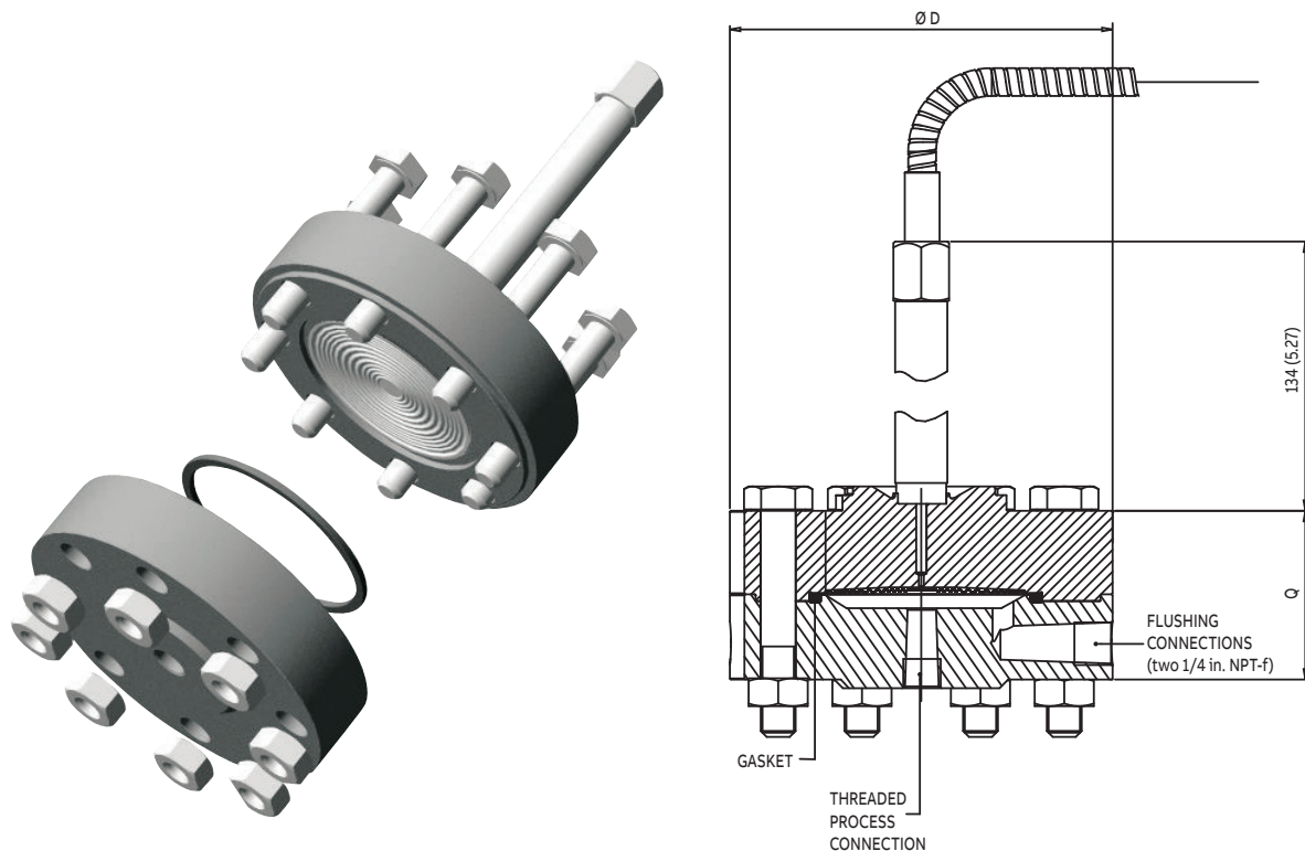
Figure 7: Off-line threaded connection diaphragm seal
