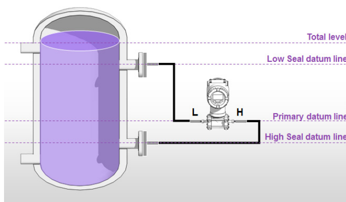
Figure 42: Density or specific gravity measurement
