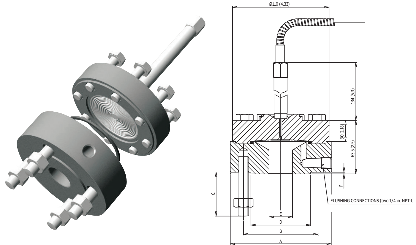
Figure 8: Off-line flanged diaphragm seal
