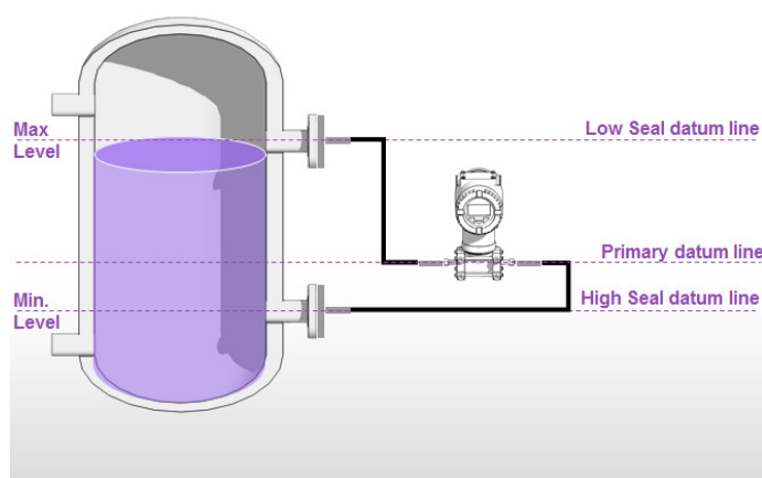
Figure 35: Level measurement of a liquid in a closed tank - pressure service only
