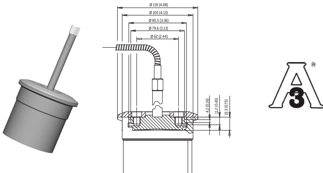
Figure 16: 4 in. Aseptic flanged connection
