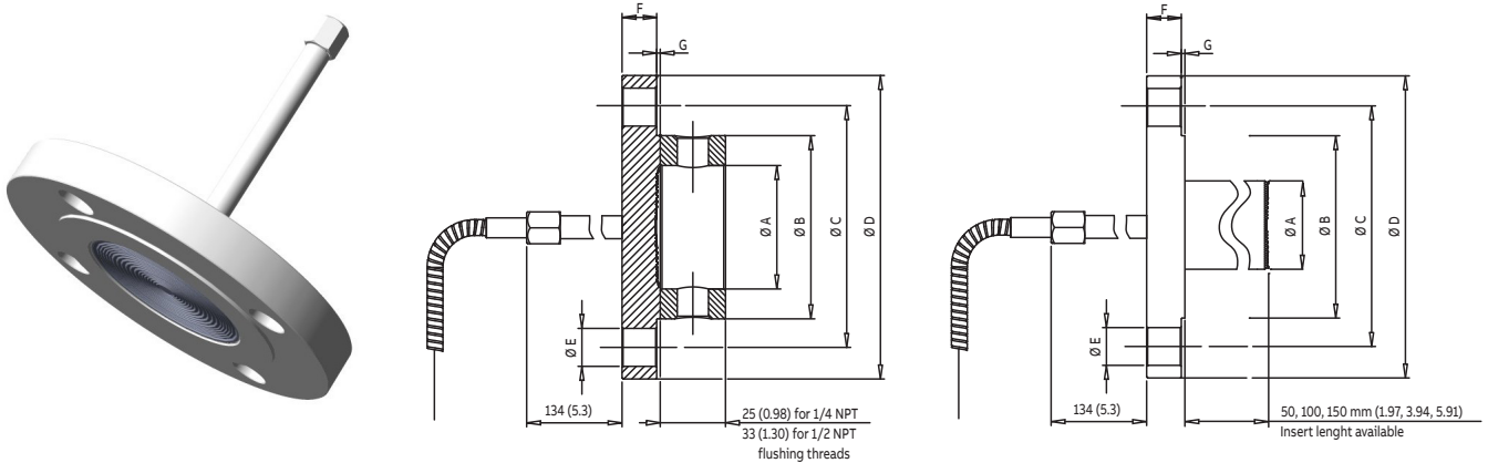
Figure 6: Fixed-flange diaphragm seal
