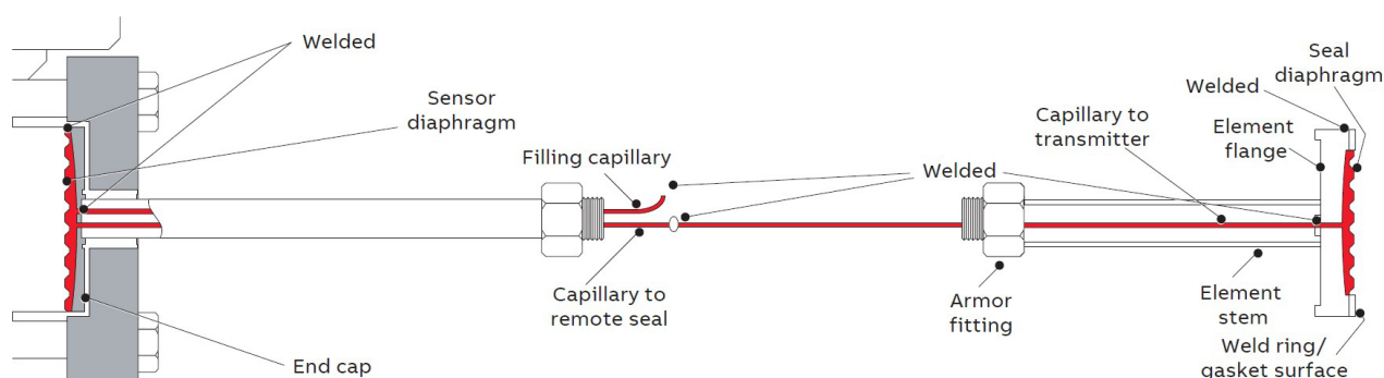
Figure 31: Seal system components
