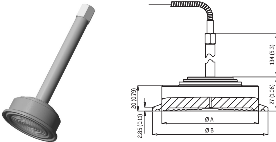
Figure 20: Triclamp sanitary seal
