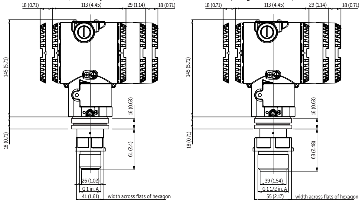
Figure 25: S26KN with GAS threaded connection
