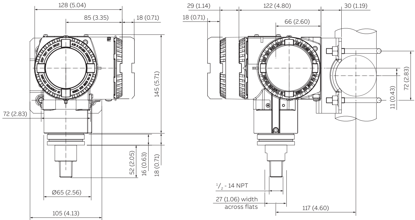
Figure 6 Transmitter with DIN aluminium housing – \frac{1}{2} in. NPT male connection for sensor E to S
