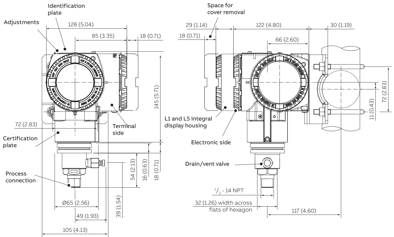
Figure 6 Transmitter with DIN aluminium housing – \frac{1}{2} in. NPT male connection for sensor E to S
