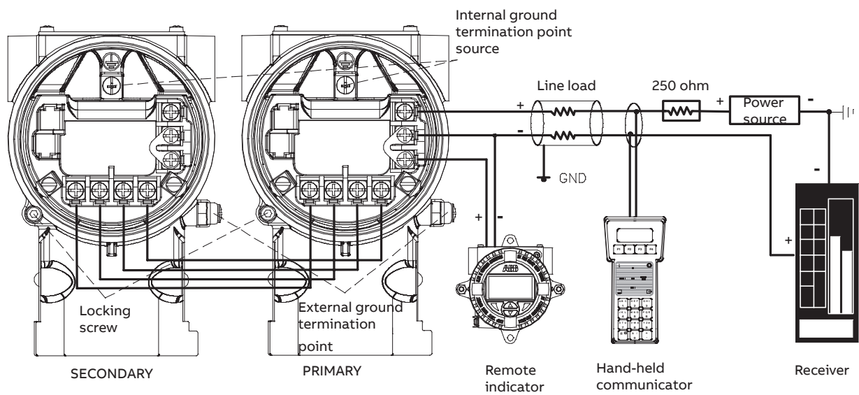
Figure 14 DDS Version
