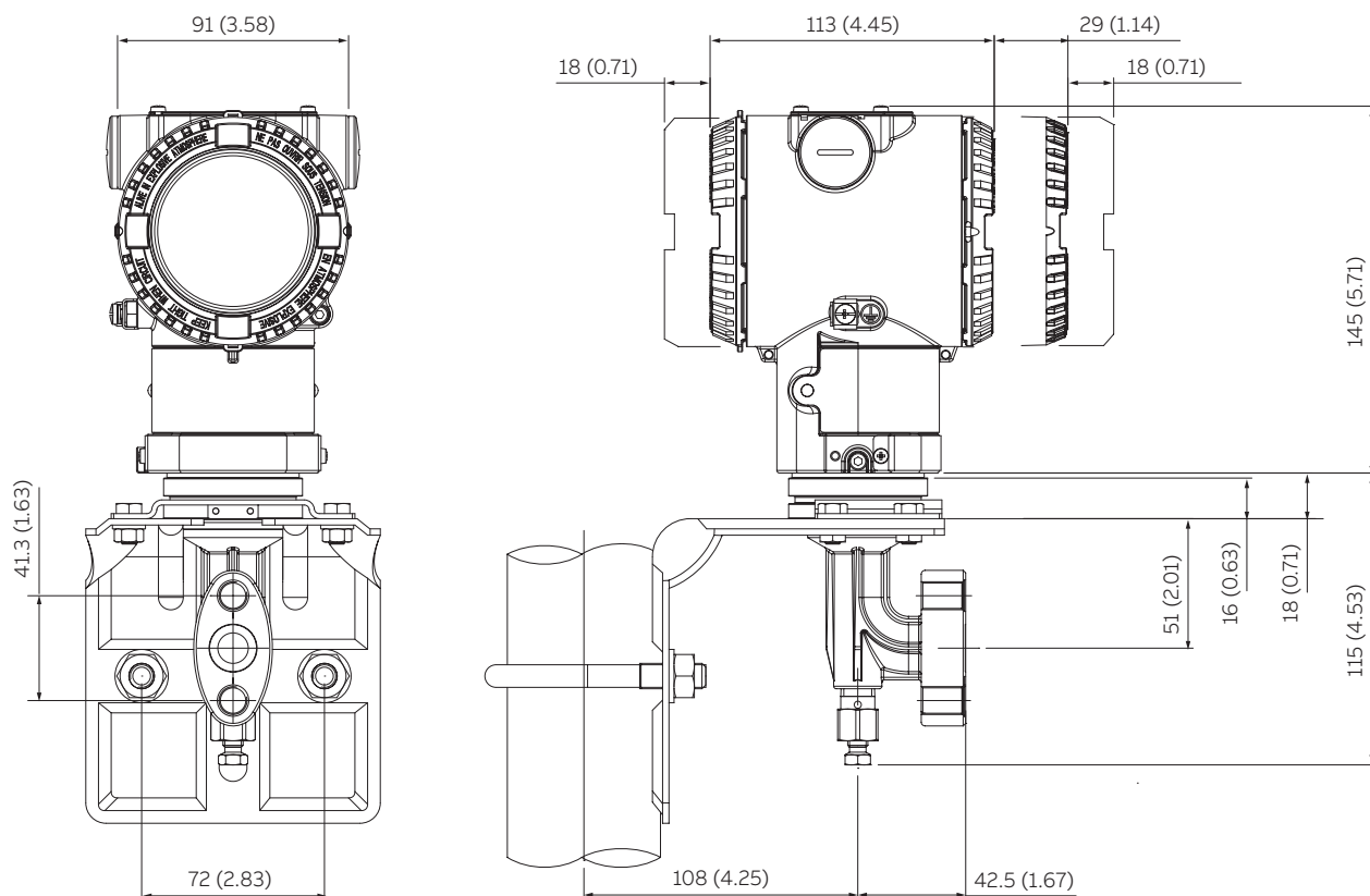
Figure 9 Transmitter with barrel housing – adapter angle (90°) entry connection for sensor E to S
