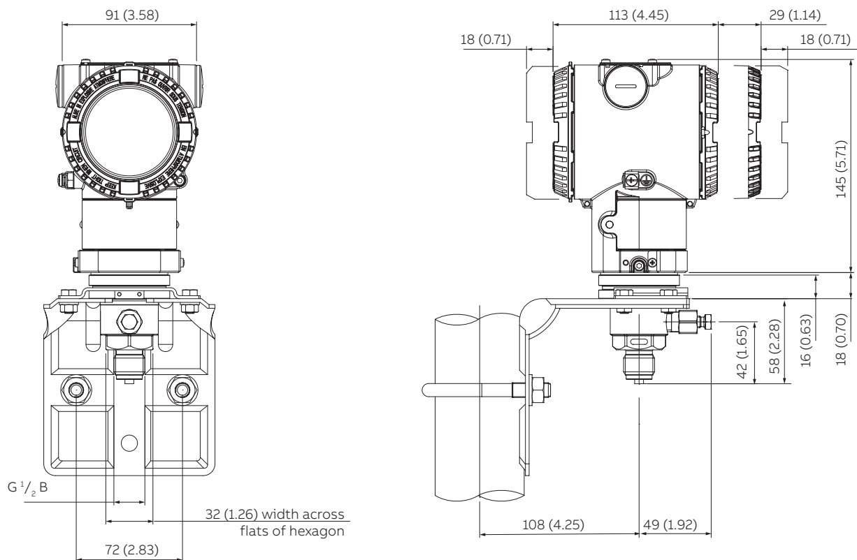
Figure 8 Transmitter with barrel housing – DIN-EN837-1 G 1/2 B connection for sensor E to S
