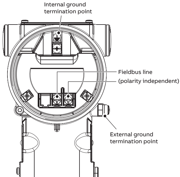
Figure 12 FIELDBUS Versions
