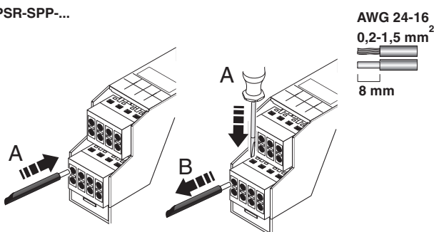
Figure 7 Connecting the cables for PSR-SPP-... (Spring-cage terminal block)
