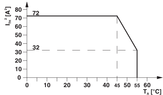
Figure 2 Derating curve - vertical or horizontal mounting position, without spacing
