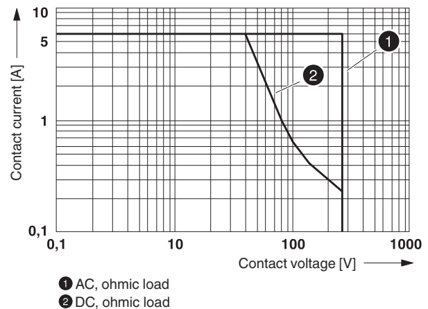
Figure 3 Relay load limit curve – ohmic load
