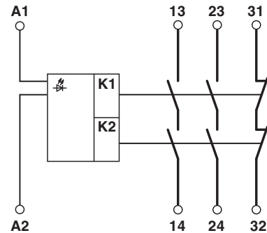
Figure 1 Block diagram
