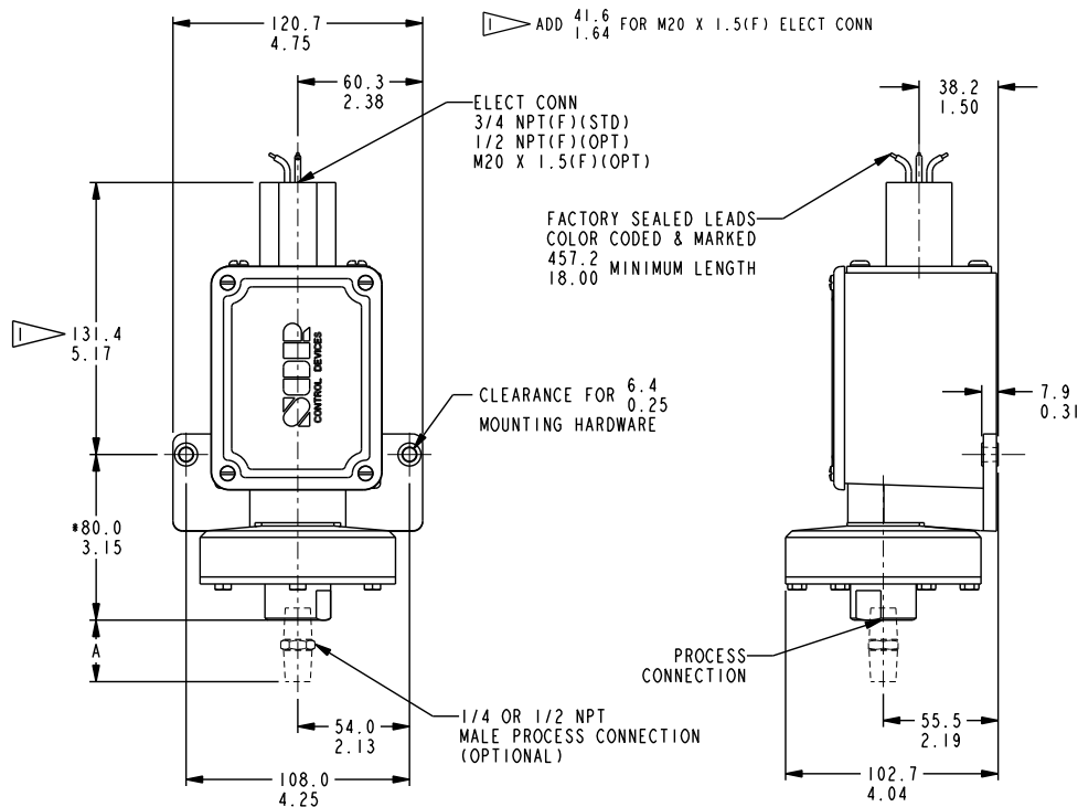
Drawing 0090177
