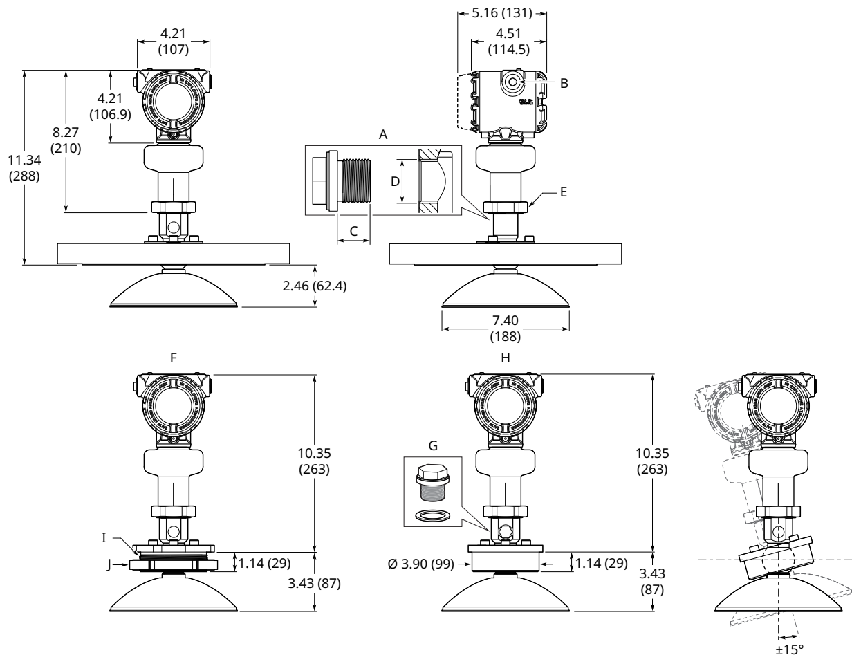
Figure 31: Parabolic Antenna
