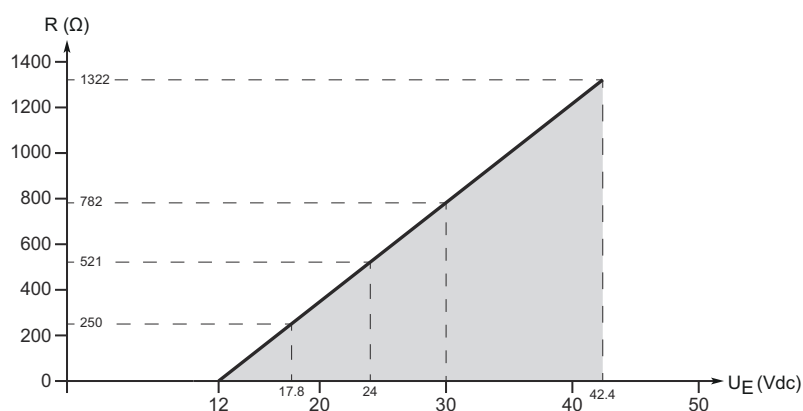
Figure 3: Load Limits
