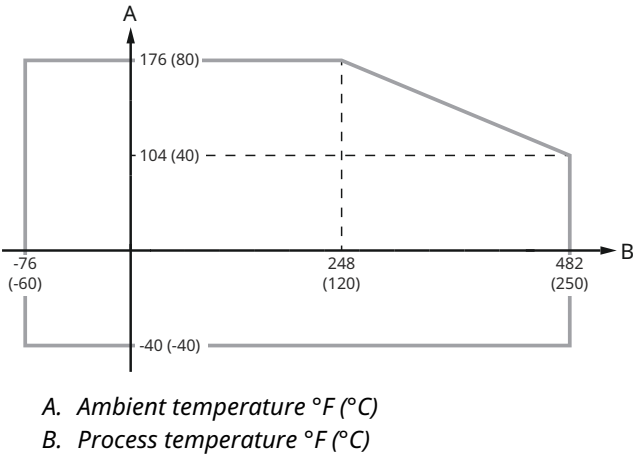
Figure 12: Ambient Temperature vs. Process Temperature
