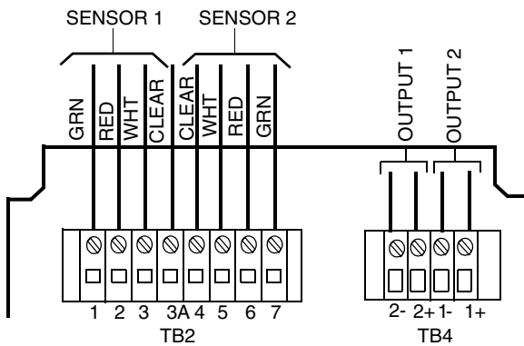
Figure 14. Metal Rear Panel Wiring - 873RS or 873CC
