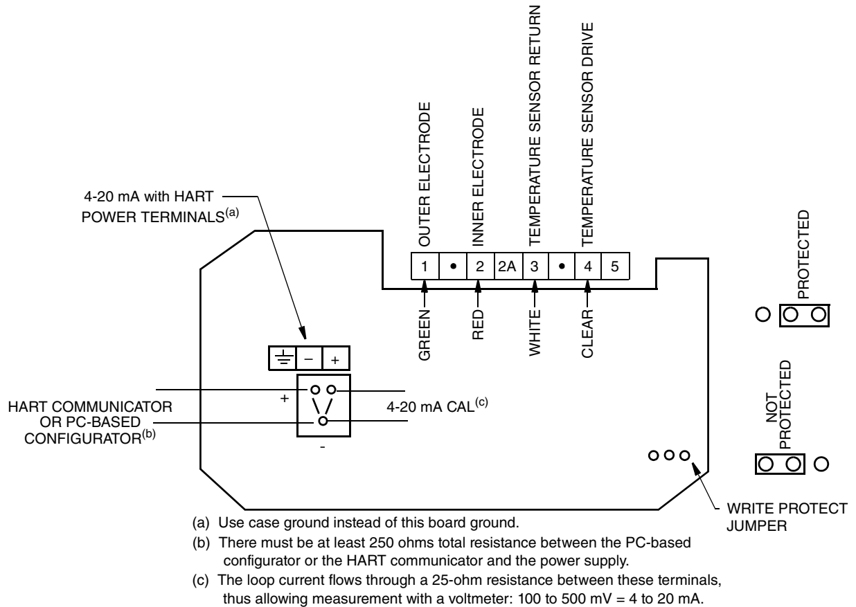
Figure 20. 876CR Wiring Connections
