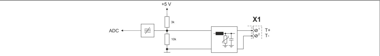
Figure 5: Temperature sensor
