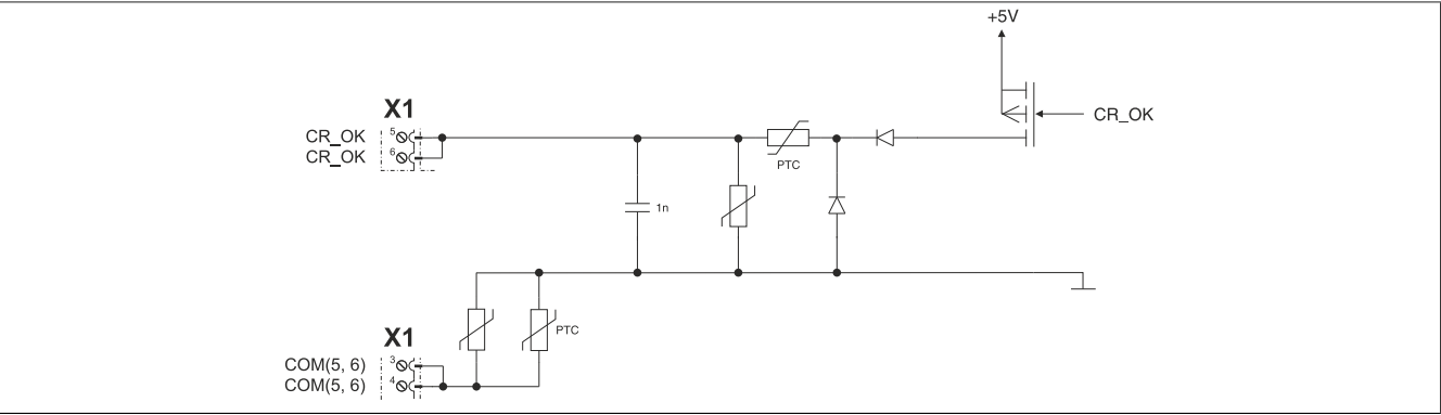
Figure 4: 8B0C - Enable
