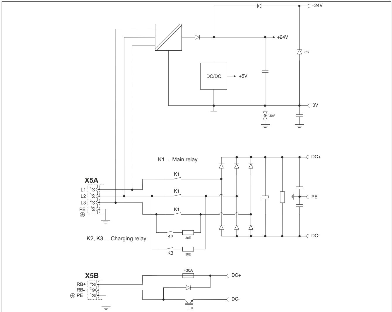
Figure 6: Power unit 8B0P0220Hx00.000-1, 8B0P0440Hx00.000-1
