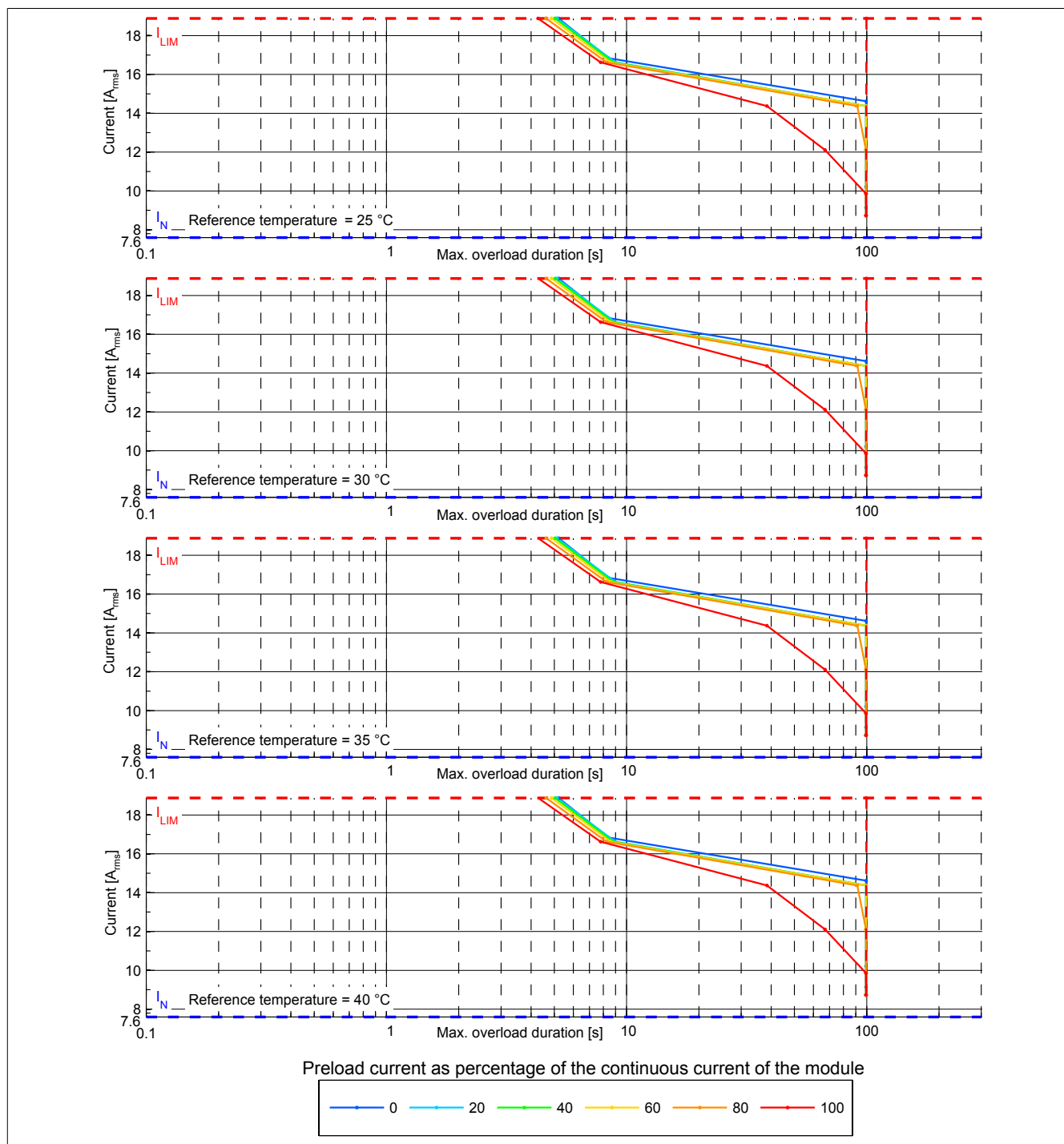
Figure 1: 8BVI0055HWDx.000-x - Overload characteristics, overload response - WARNING
