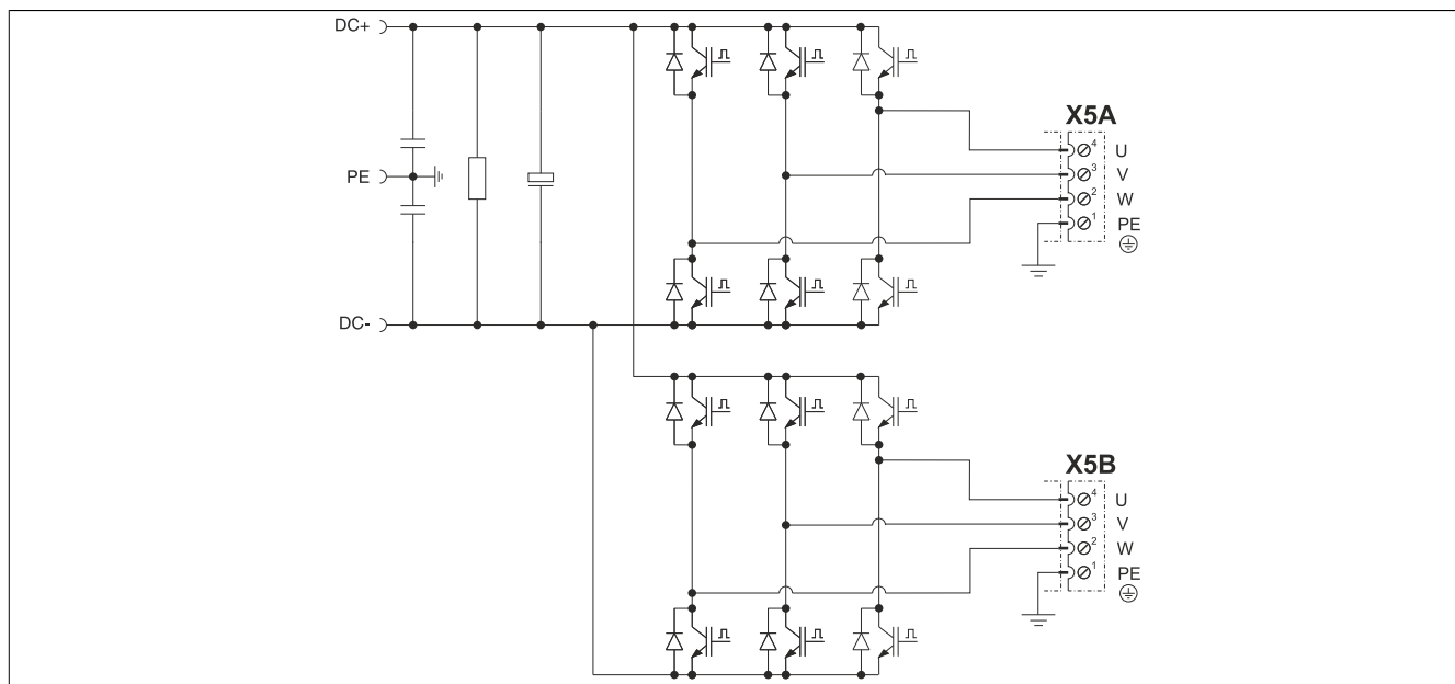
Figure 9: Motor
