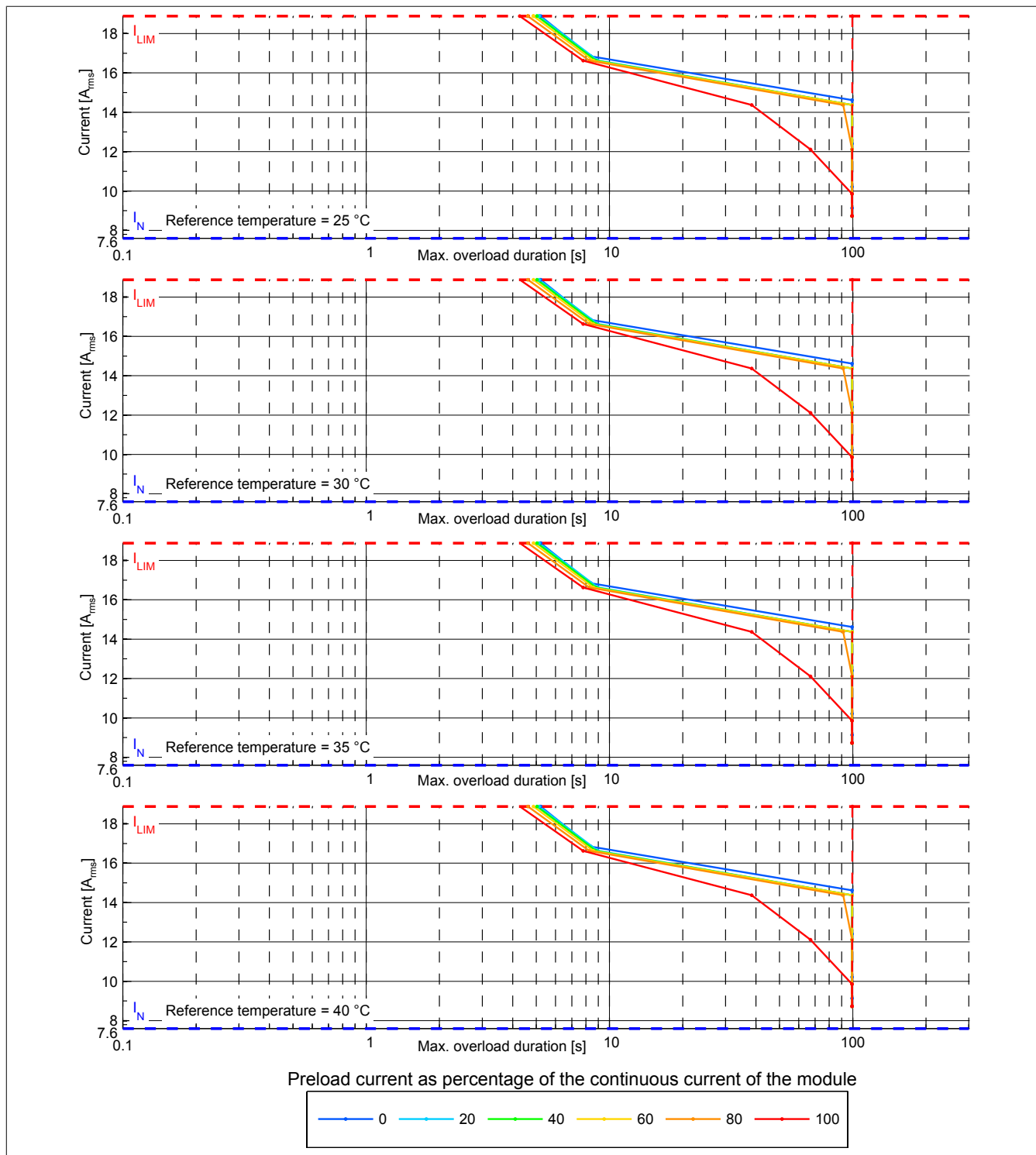
Figure 2: 8BVI0055HWDx.000-x - Overload characteristics, overload response - ERROR + STOP
