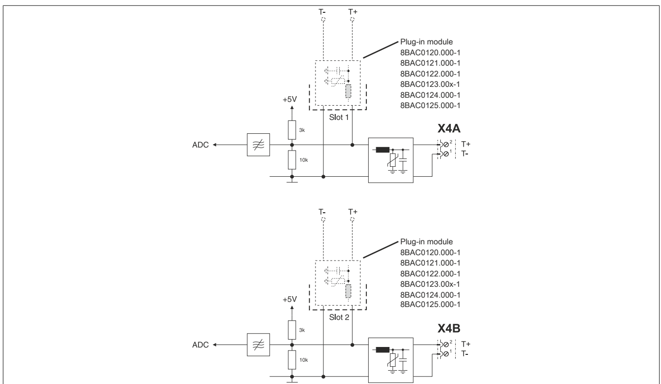
Figure 8: Temperature sensor
