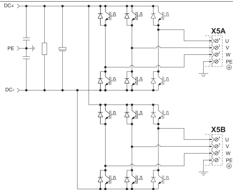
Figure 12: Motor
