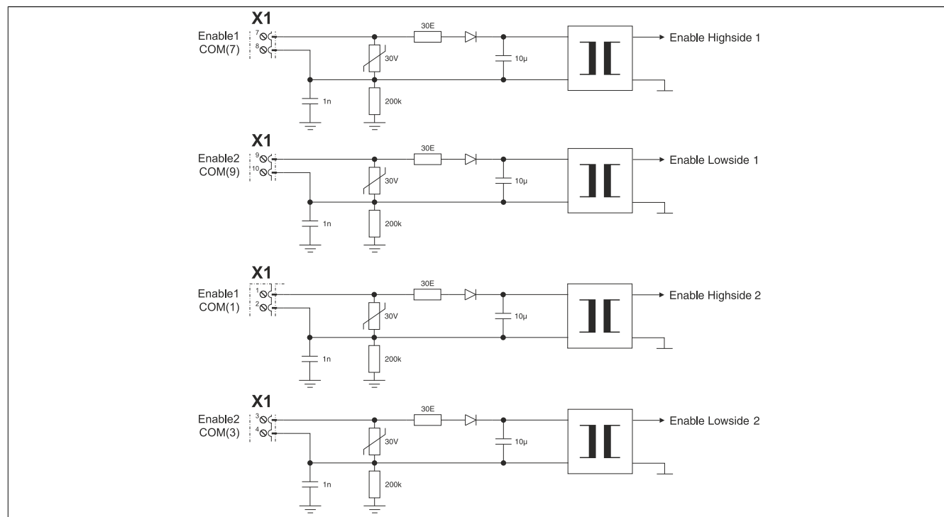
Figure 7: Enable
