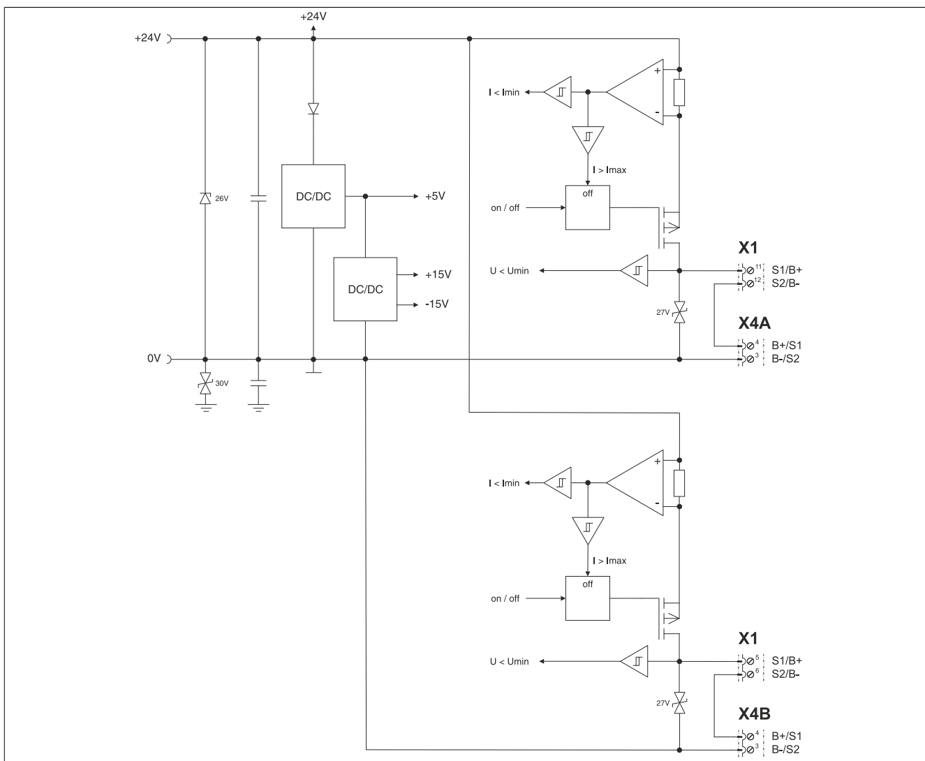
Figure 10: Holding brake
