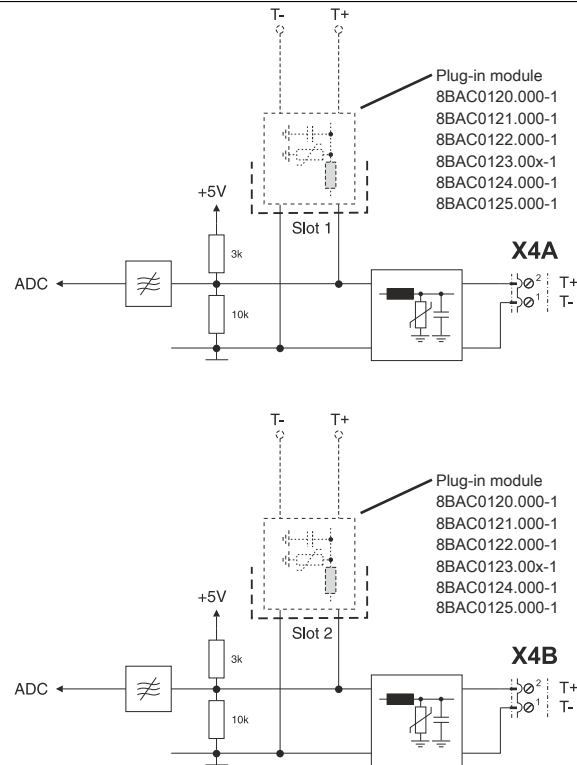
Figure 11: Temperature sensor
