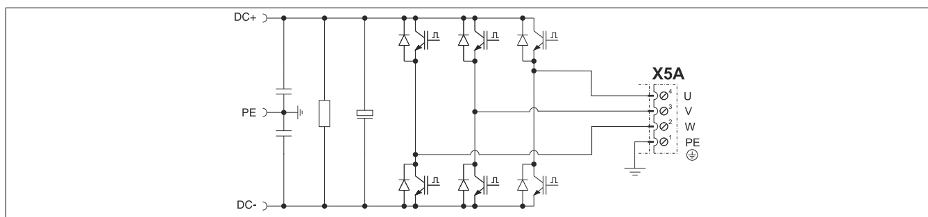
Figure 12: Motor
