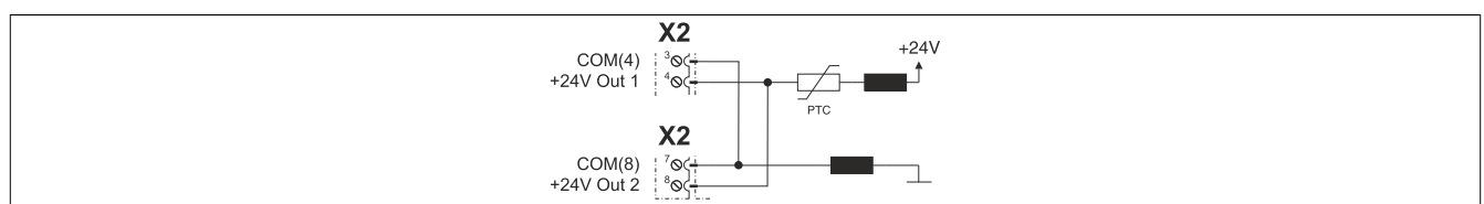
Figure 9: 24 VDC out
