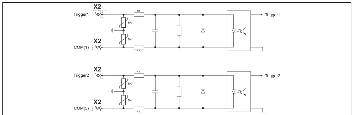
Figure 8: Trigger inputs
