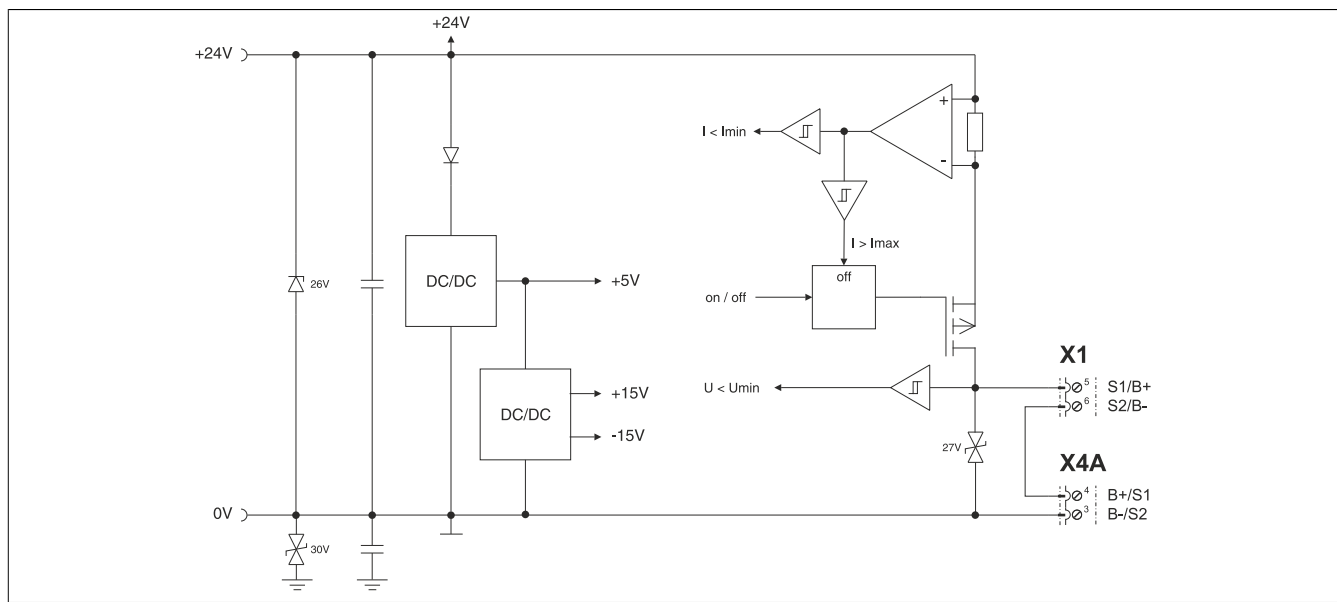
Figure 10: Holding brake
