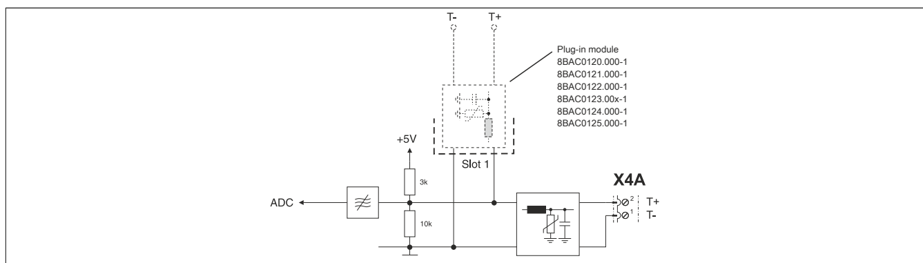
Figure 11: Temperature sensor
