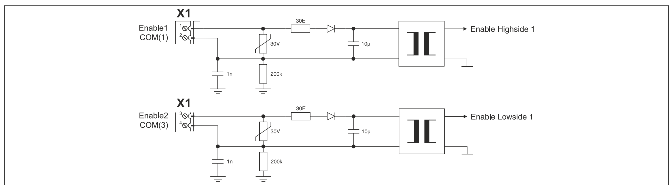
Figure 7: Enable
