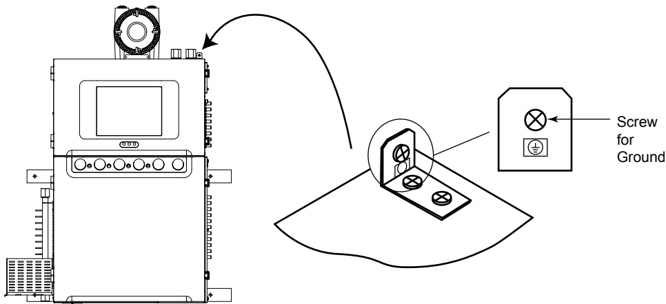
Figure 2.22 Earth terminal for the GC8000
