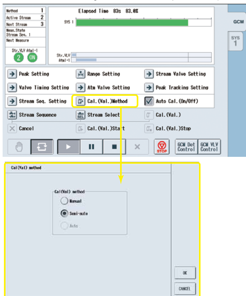
Figure 1.28 An example of the calibration (validation) method window on the GCM operation status screen on the GC-HMI analyzer operation display
