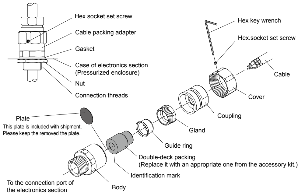
Figure 2.17 Procedure for mounting a cable packing adapter for the electronics section
