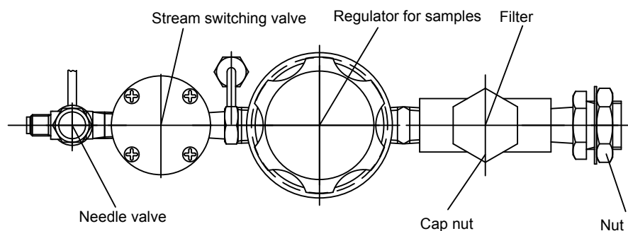
Figure 6.44 Example of Sample Processing System (May contain a Stop Valve depending on the system)
