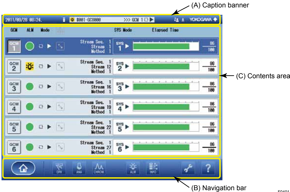
Figure 4.1 Screen Layout
