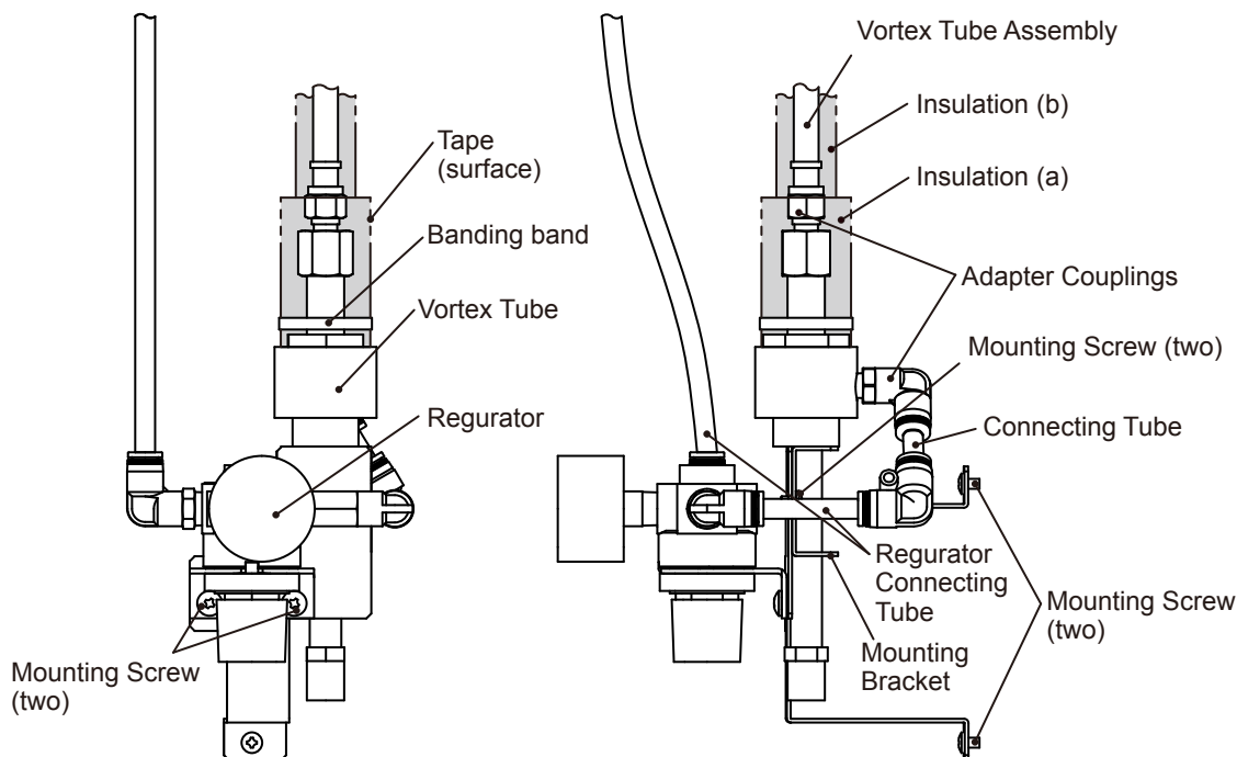
Figure 6.24 Vortex Tube
