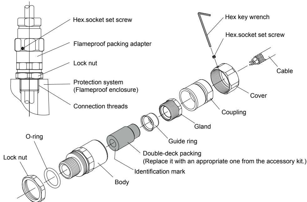
Figure 2.16 Procedure for mounting a cable packing adapter for a protection system
