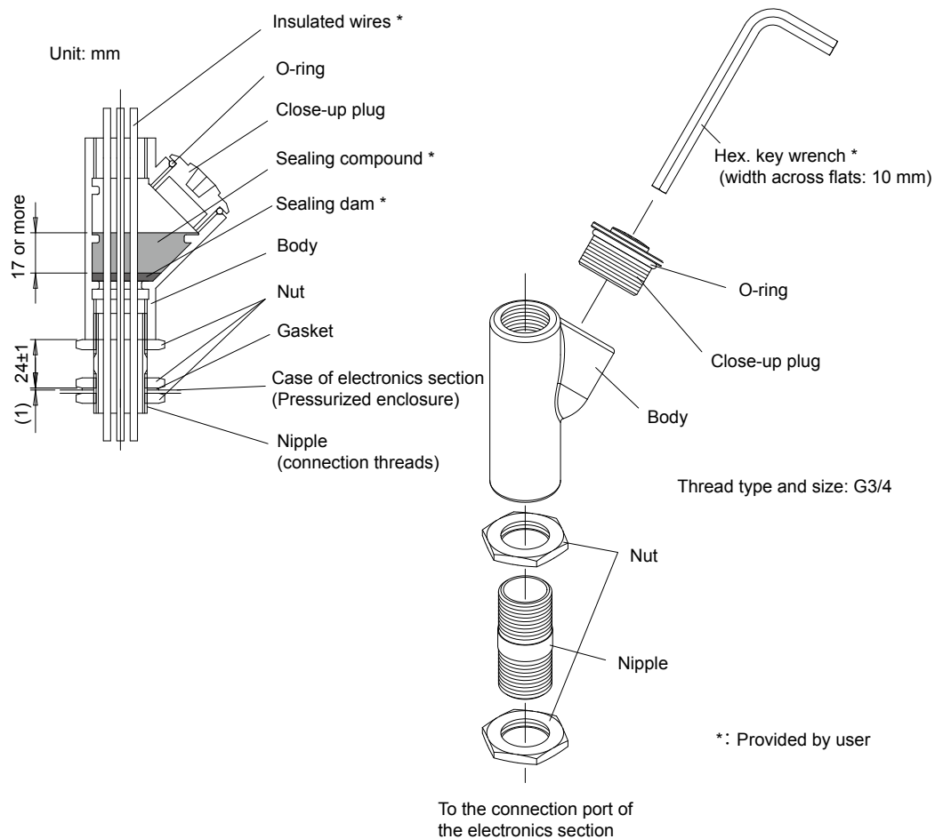
Figure 2.18 Mounting procedure for sealing fitting (accessory)
