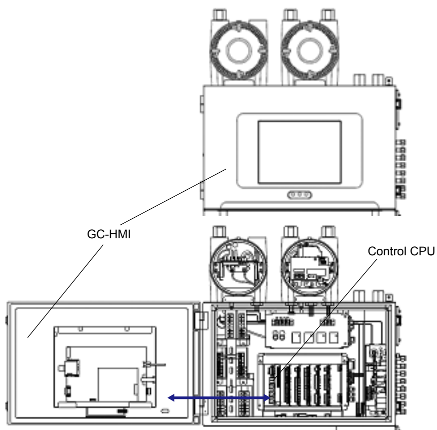
Figure 1.12 Position of the GC-HMI (touch panel) of the analyzer and control CPU
