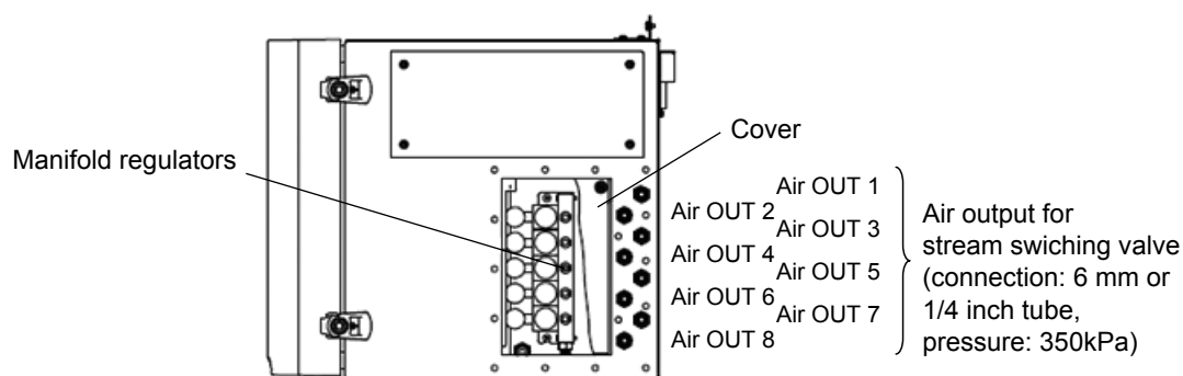
Figure 1.6 Pressure control section of the control unit
