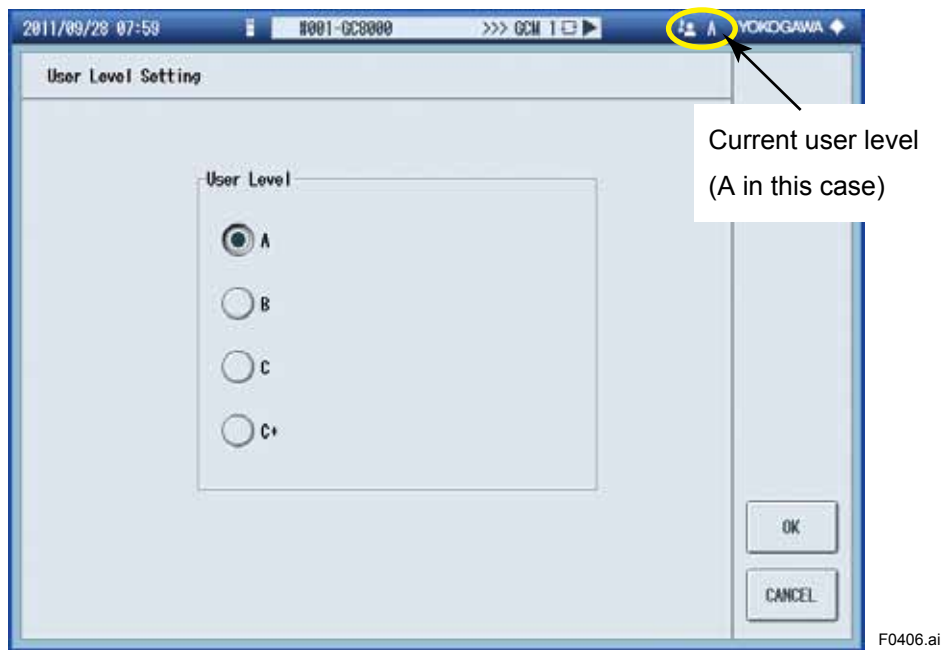
Figure 4.6 User Level
