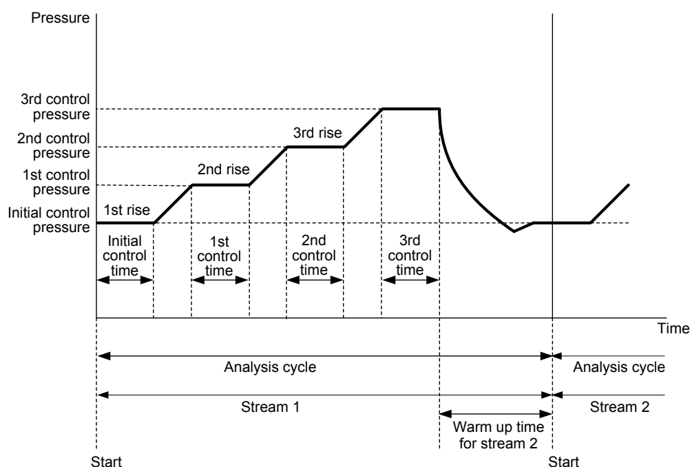
Figure 1.39 EPC program operations
