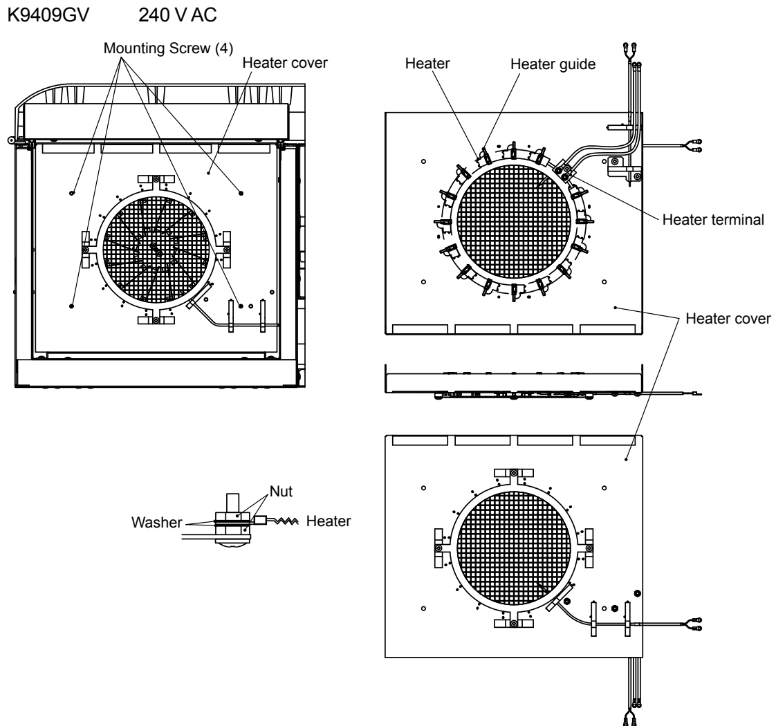
Figure 6.26 Heater for Isothermal Oven
