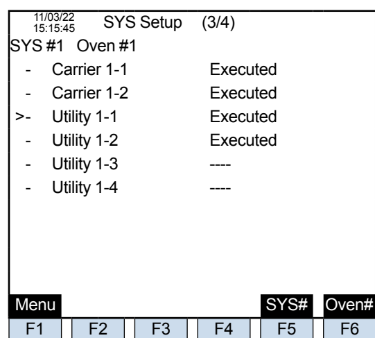
Figure 1.40 Setting example of SYS (GC-HMI EtherLCD)
