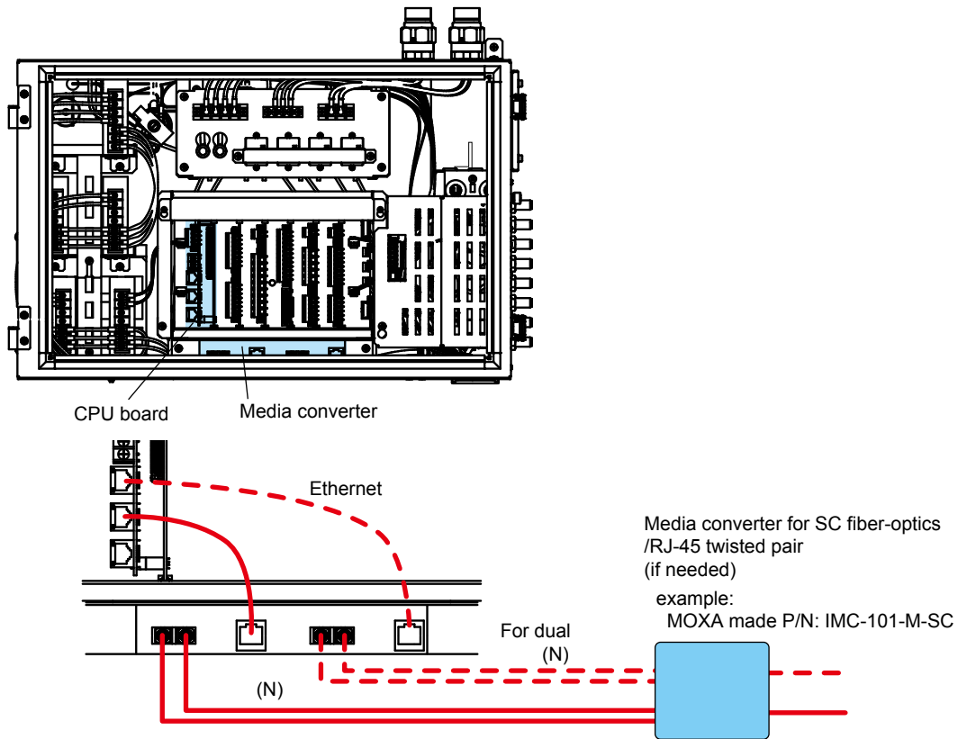
Figure 2.25 Ethernet (optical fiber)
