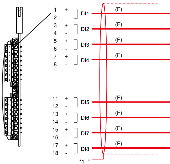
Figure 2.33 Wiring for a contact input card
