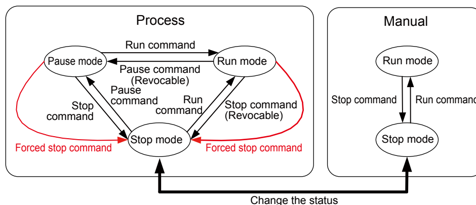
Figure 1.16 Diagram of Changing the Status and Operation Modes
