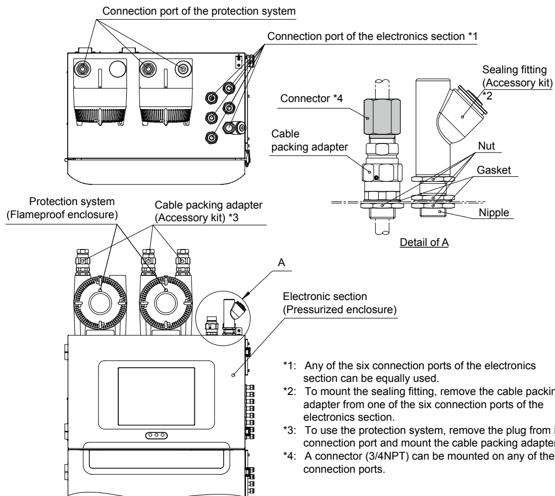
Figure 2.15 Wiring in TIIS specification
