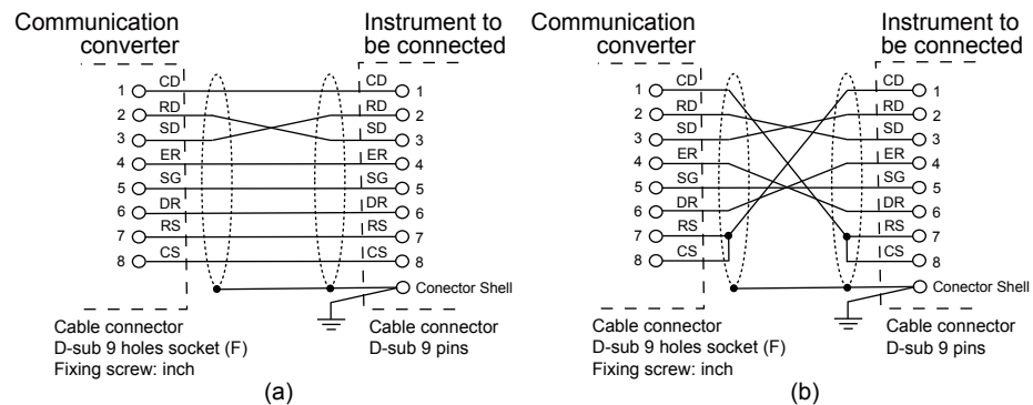
Figure2.28 Wiring for serial communication cards
