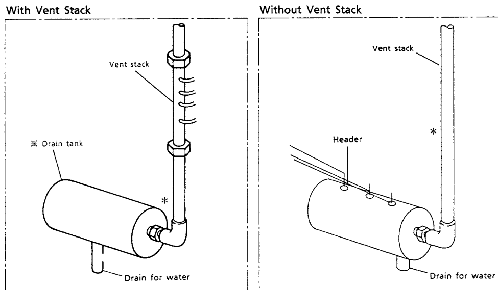
Figure 2.4 Example of vent stack installation
