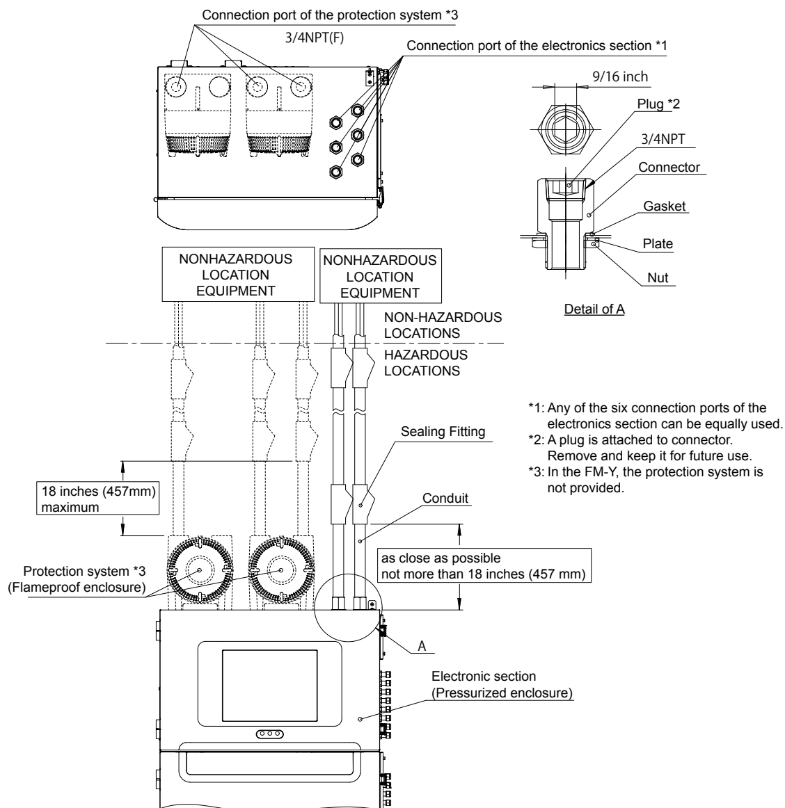
Figure 2.12 Wiring in FM specification
