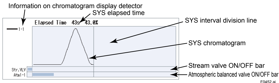
Figure 4.52 Example of SYS Chromatogram Display Area
