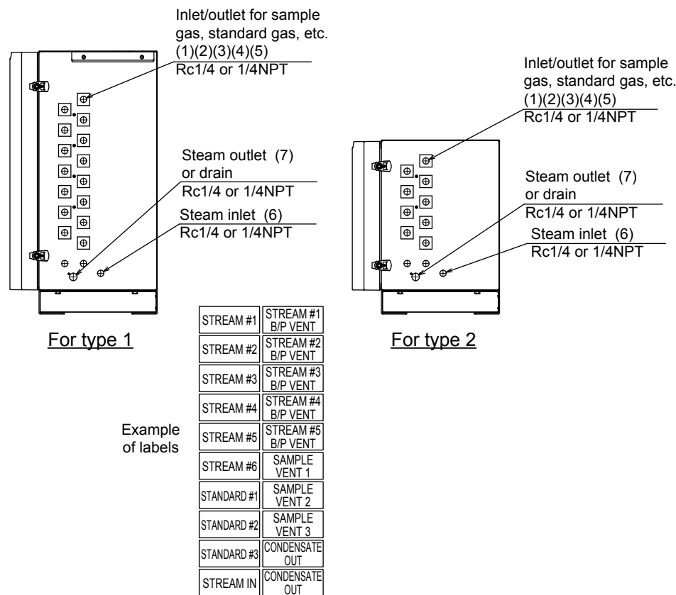
Figure 2.9 Analyzer base sampling unit (GCSMP)
