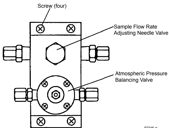
Figure 6.46 Atmospheric Pressure Balancing Valve and Sample Flow Rate Adjusting Needle Valve
