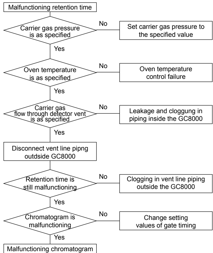
Figure 7.3 Troubleshooting Diagram for Malfunctioning Retention Time
