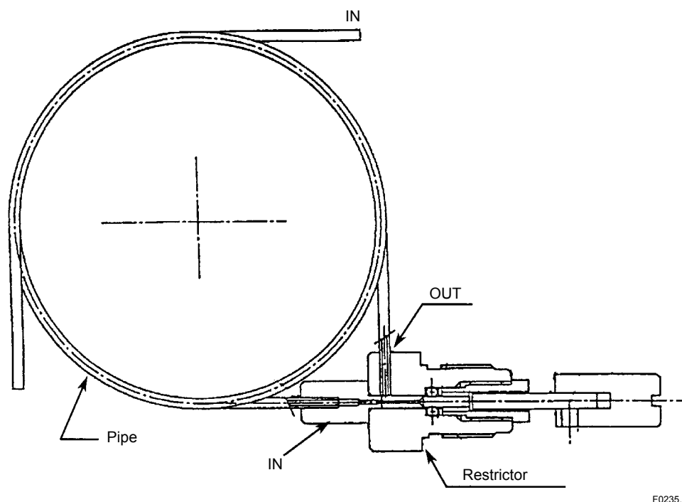
Figure 6.35 Restrictor
