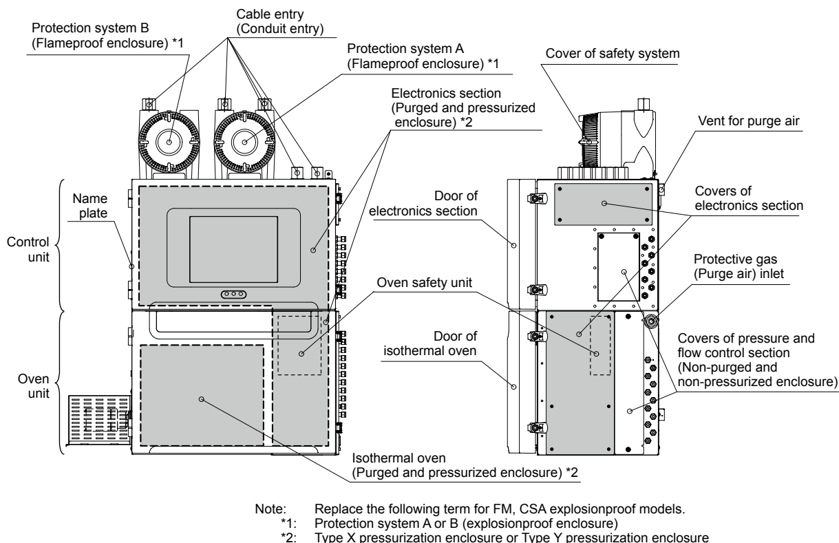
Figure 2 Analyzer component names for explosionproof type
