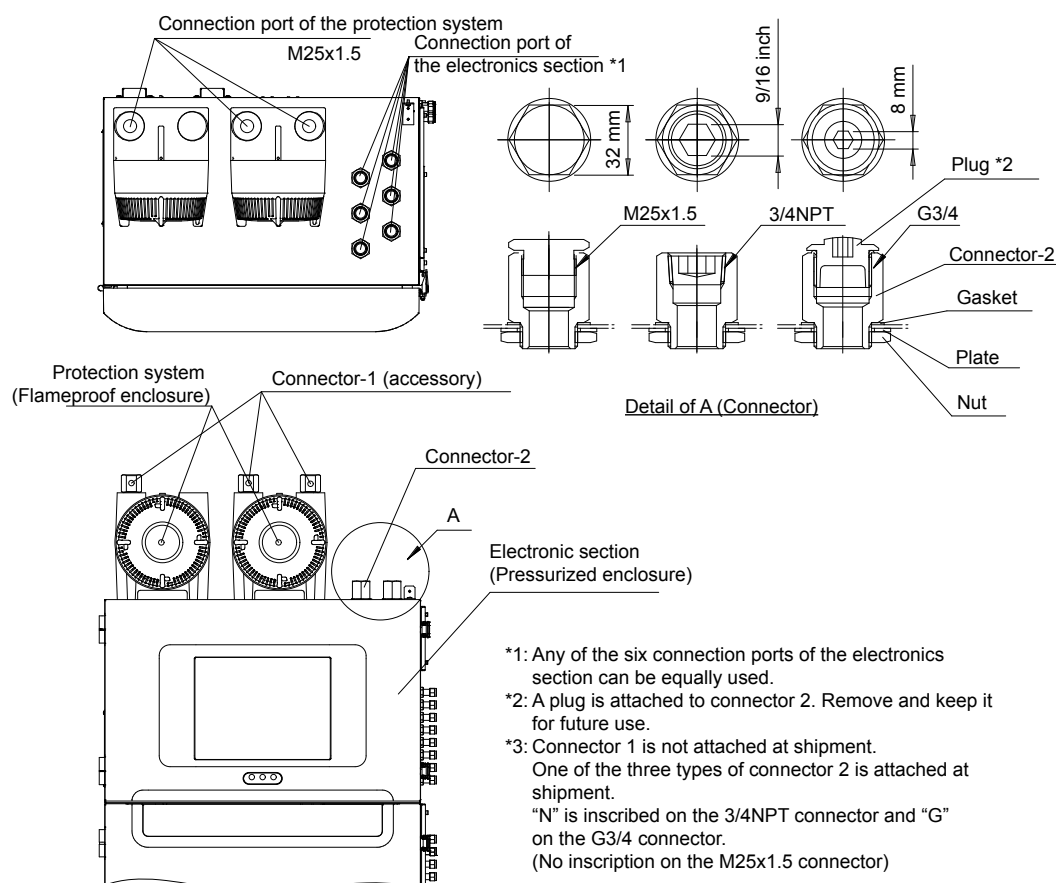
Figure 2.14 Wiring in ATEX or IECEx specification
