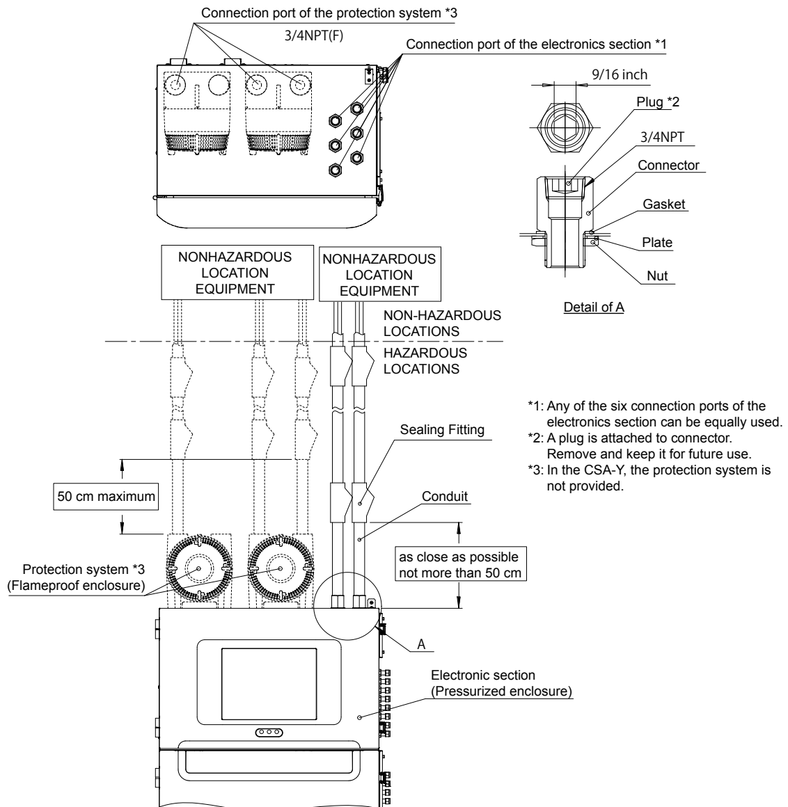
Figure 2.13 Wiring in CSA specification
