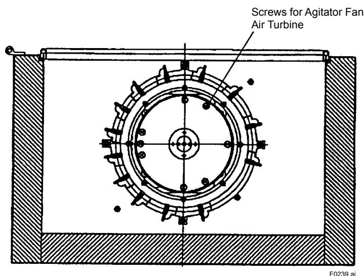
Figure 6.39 Air Turbine for Agitator Fan
