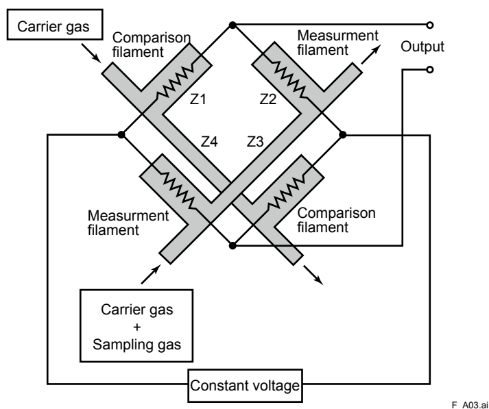
Figure 3 Fundamental Principle of Thermal Conductivity Detector
