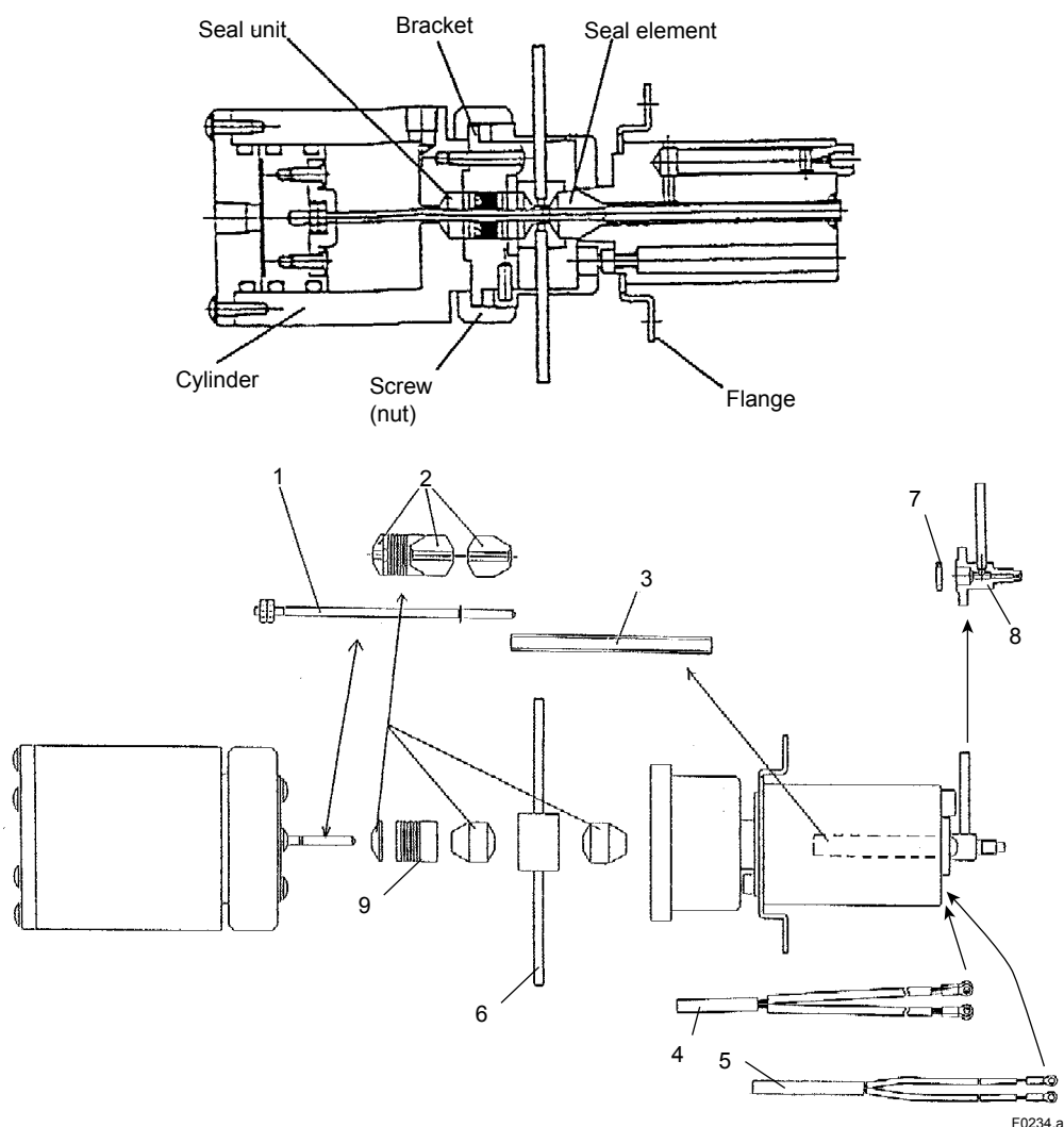
Figure 6.34 Liquid Sampling Valve (LSV)
