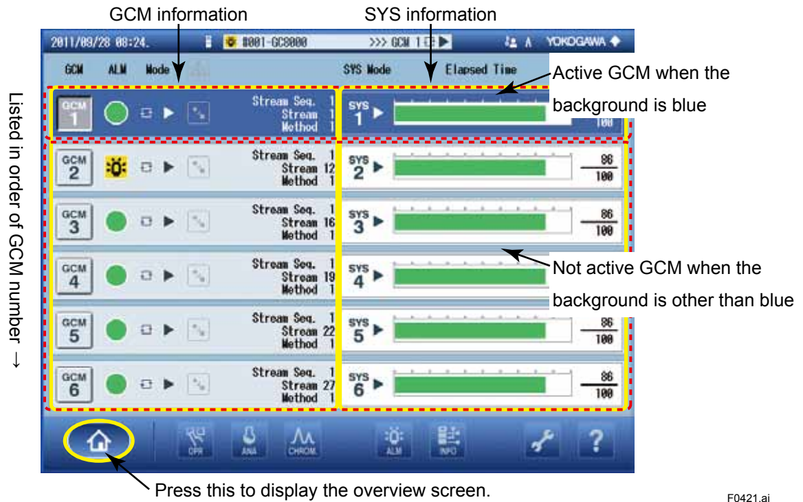
Figure 4.21 Example of Overview Screen
