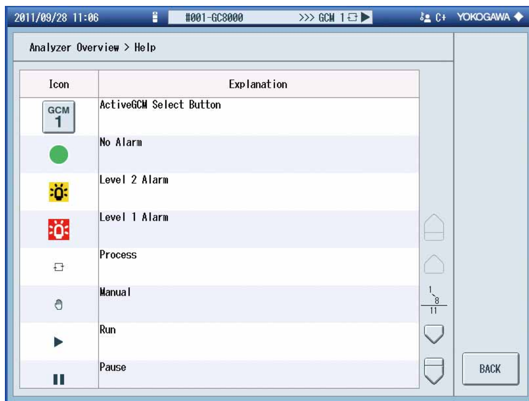
Figure 4.86 Example of Help Screen (Analyzer Overview Screen)
