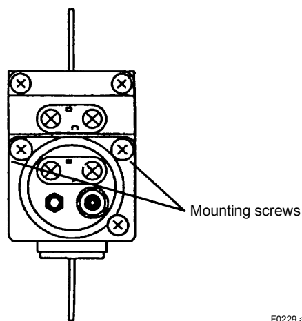
Figure 6.29 FID
