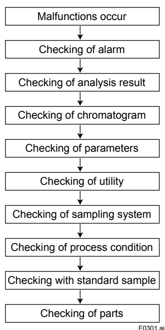
Figure 7.1 Common Procedure of Troubleshooting
