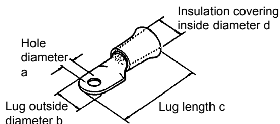
Figure 2.19 Crimp-on terminal
