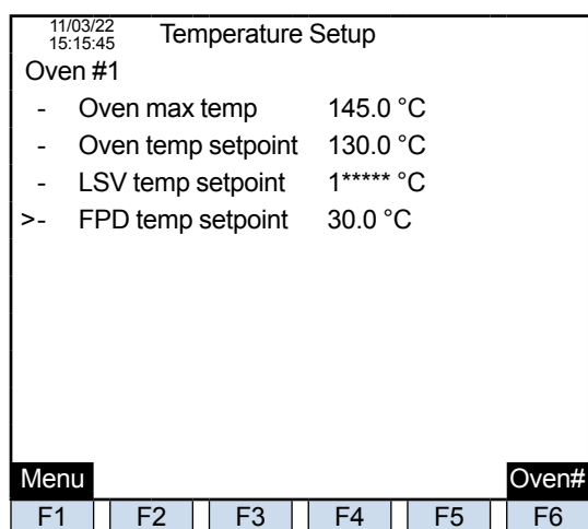
Figure 1.11 Example of the operation condition configuration screen of the GC-HMI (touch panel) EtherLCD
