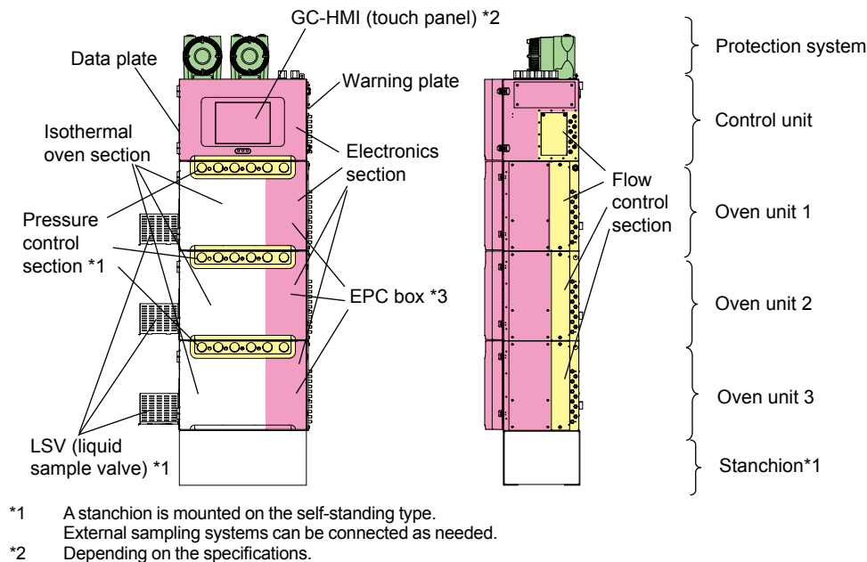
Figure 1.5 Structure and components of Type 3
