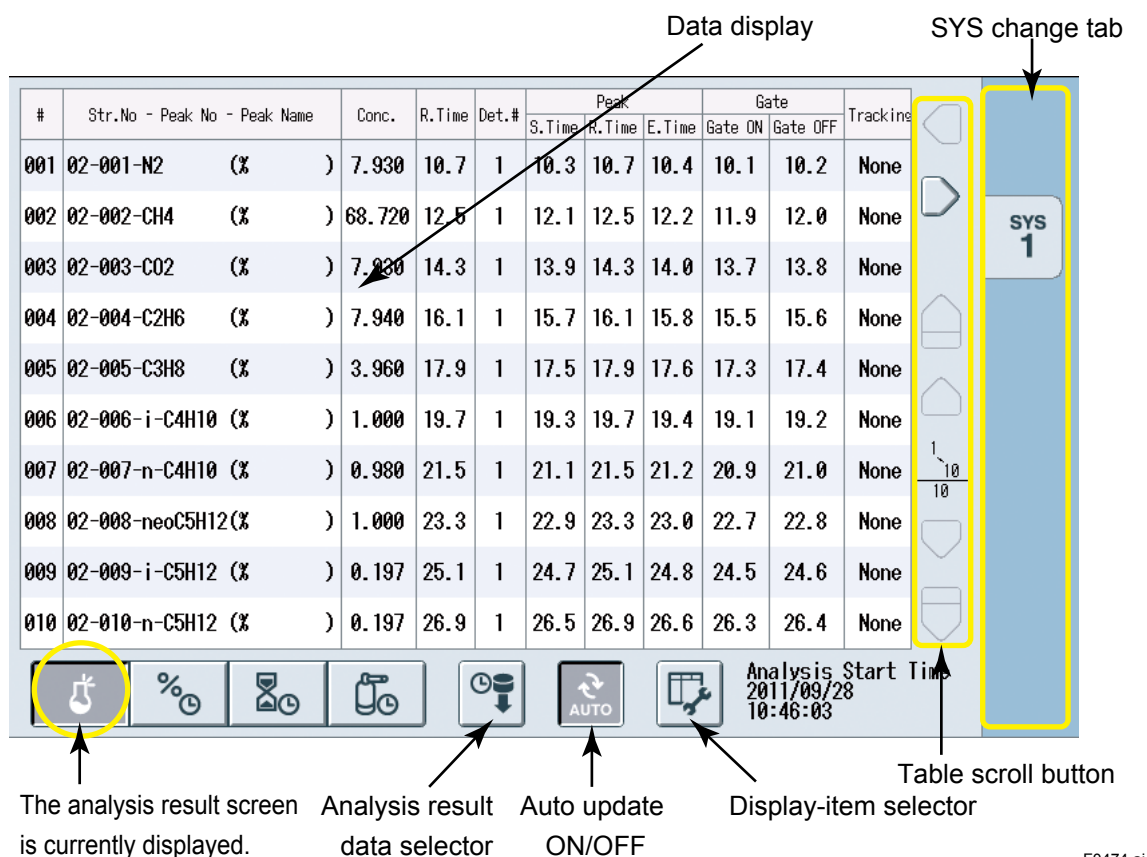
Figure 4.74 Analysis Result Screen Layout
