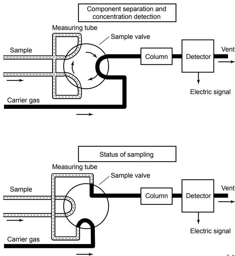
Figure 1 Basic Configuration of Gas Chromatograph
