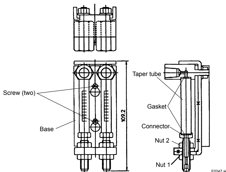
Figure 6.47 Taper Tube
