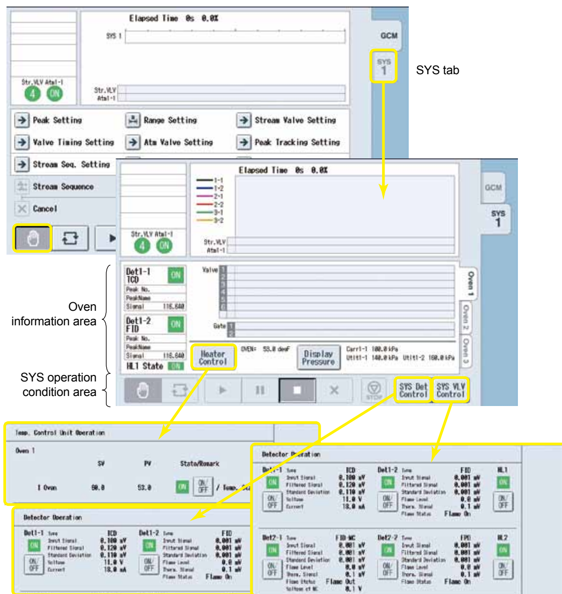
Figure 1.34 Operation examples of the temperature regulator control window and others on the GC-HMI analyzer operation display
