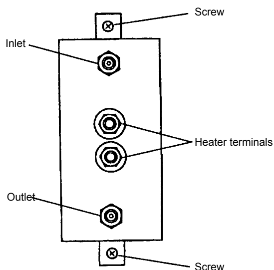
Figure 6.30 Methanizer
