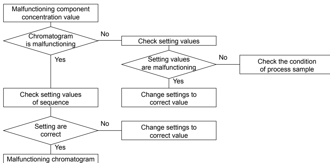
Figure 7.2 Troubleshooting Diagram for Malfunctioning Component Concentration Value
