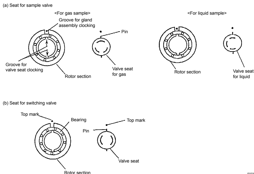
Figure 6.33 Valve Seat
