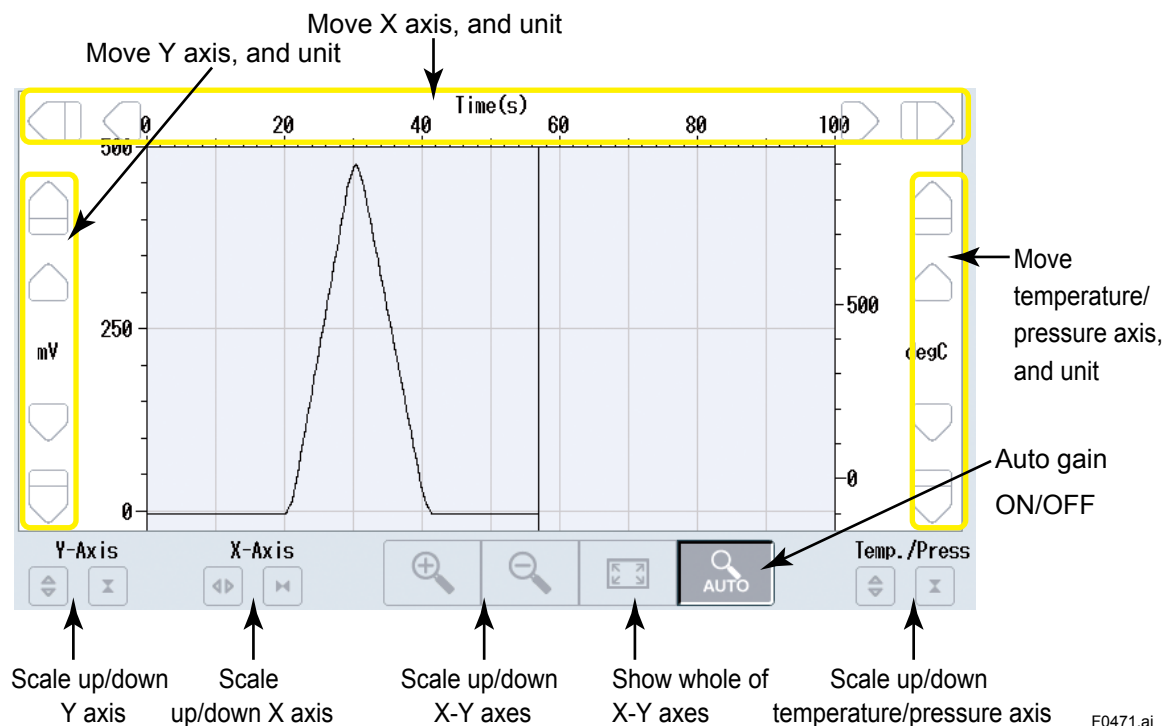
Figure 4.71 Example of Zoomed View
