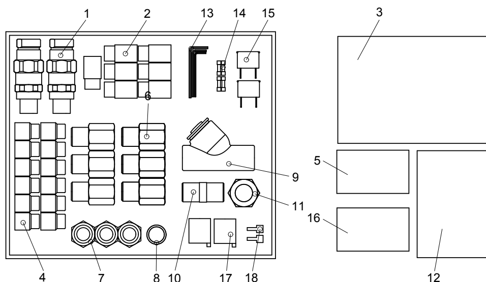
Figure 2.2 Accessory kit
