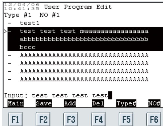
Figure 5.38 User program edit screen (Example of editing 6)
