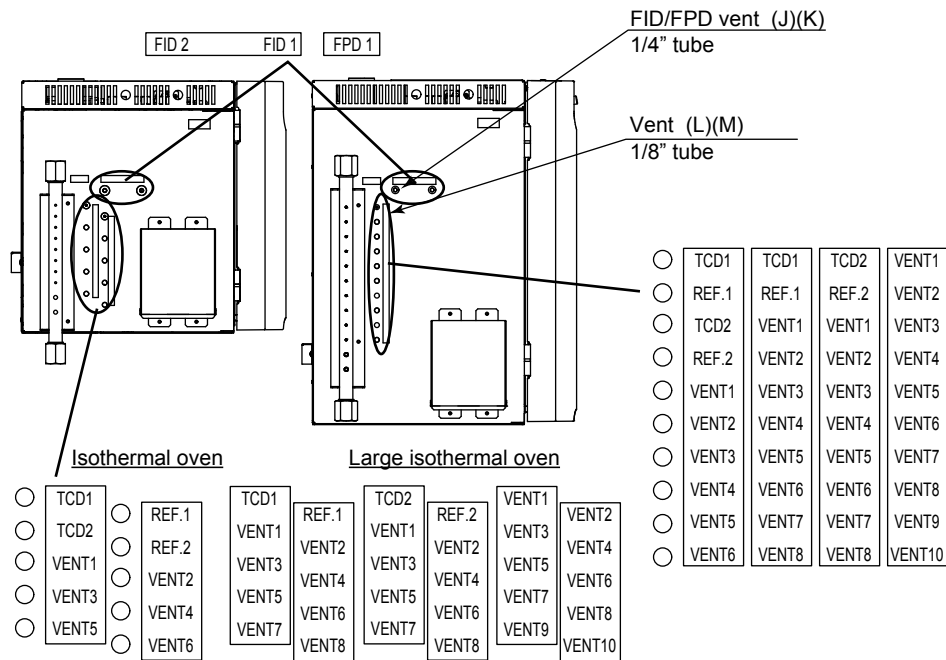
Figure 2.8 Left side of isothermal oven and large isothermal oven
