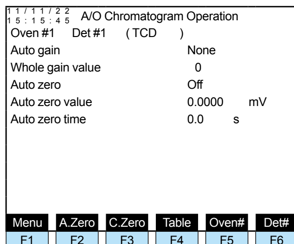
Figure 5.26 Example of the A/O chromatogram operation screen
