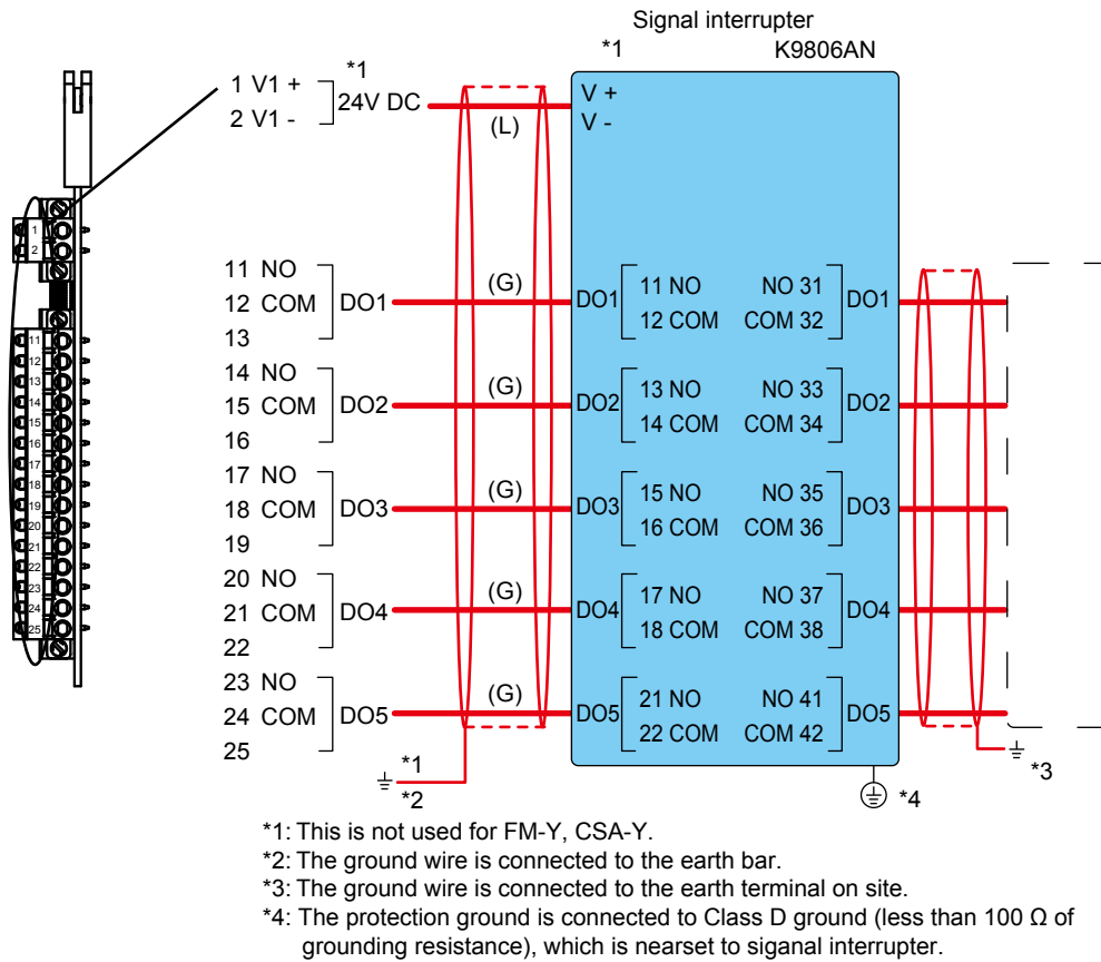
Figure 2.31 Wiring for a contact output card
