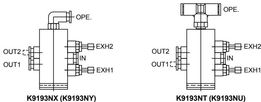
Figure 6.49 Pneumatic Valve for Actuating External Air Supply
