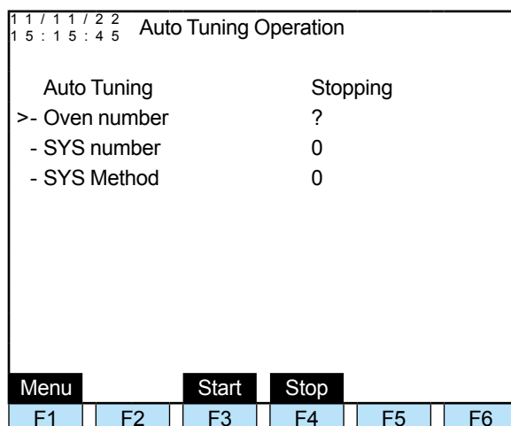
Figure 5.43 Example of the auto tuning operation screen
