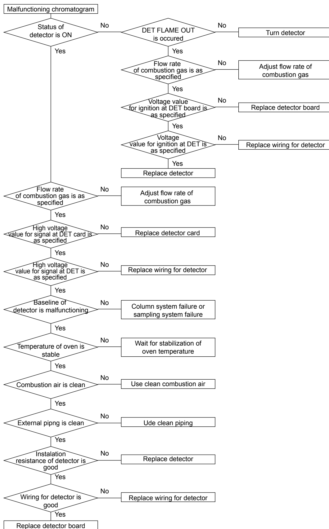
Figure 7.5 Troubleshooting Diagram for Malfunctioning Chromatogram (FID)
