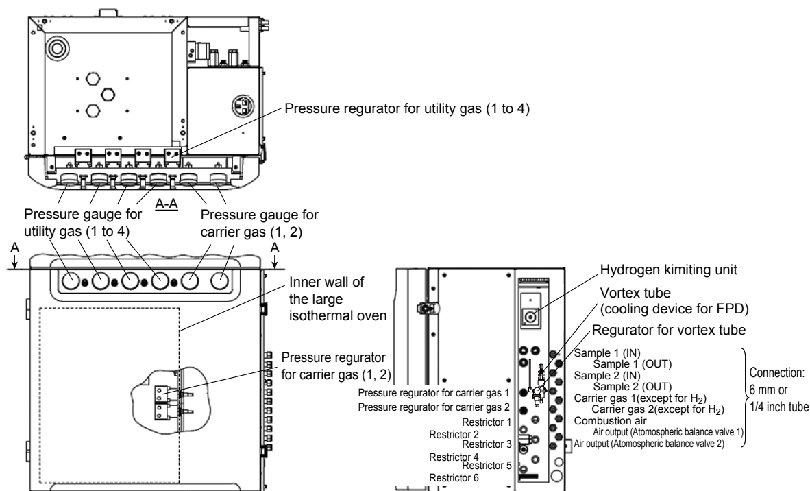
Figure 1.8 Pressure and flow control section of the large isothermal oven
