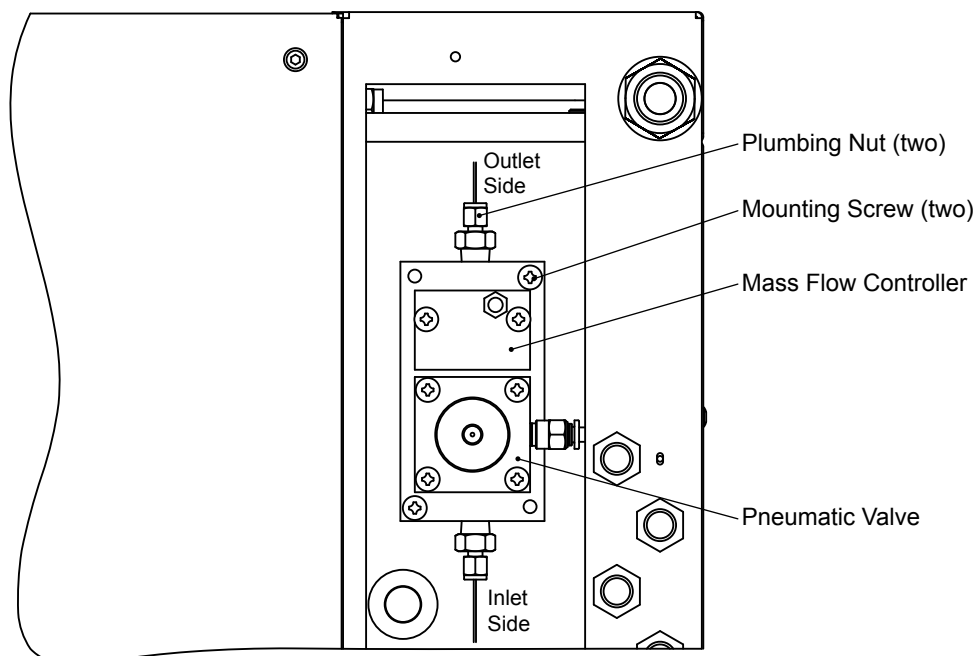
Figure 6.25 Hydrogen Limiting Unit
