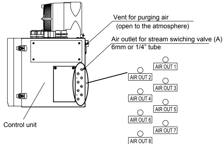
Figure 2.6 Right side of control unit
