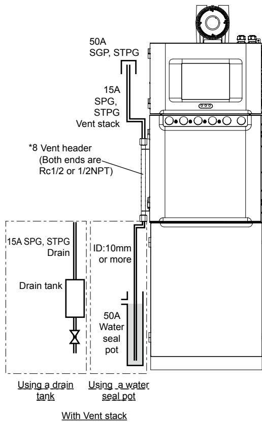
Figure 2.4 Example of vent stack installation
