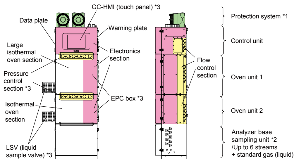
Figure 1.3 Structure and components of Type 1
