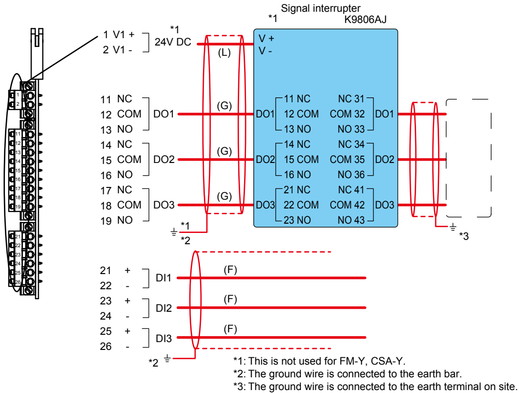
Figure 2.35 Wiring for a contact input/output card
