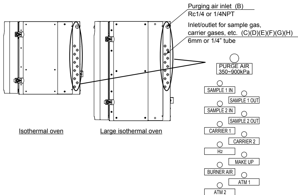
Figure 2.7 Left side of isothermal oven and large isothermal oven
