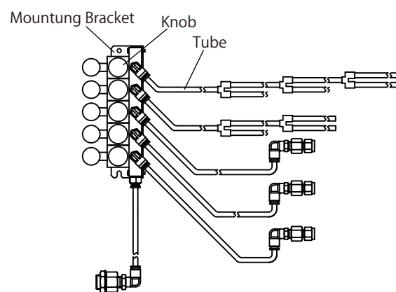
Figure 6.21 Regulator for Purge Air and Solenoid-Valve Air
