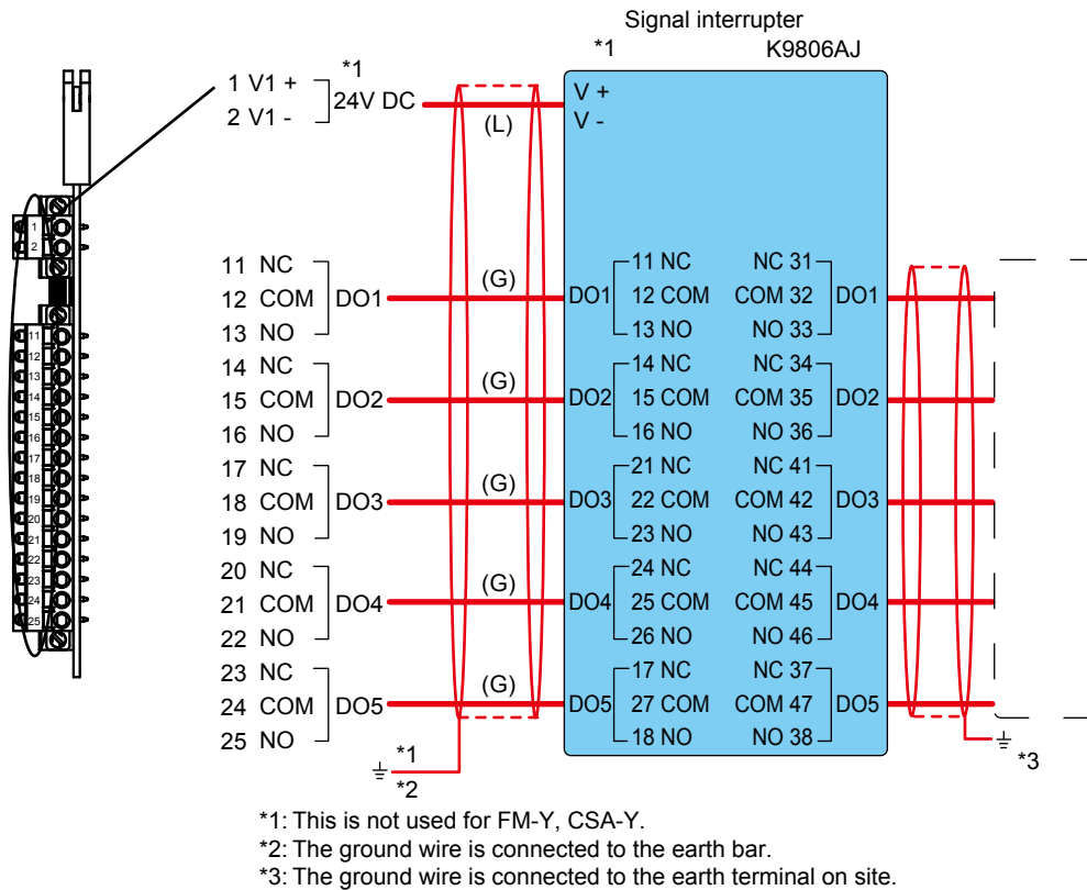
Figure 2.32 Wiring for a contact output card
