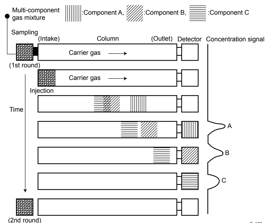
Figure 2 Separating Components Using a Column
