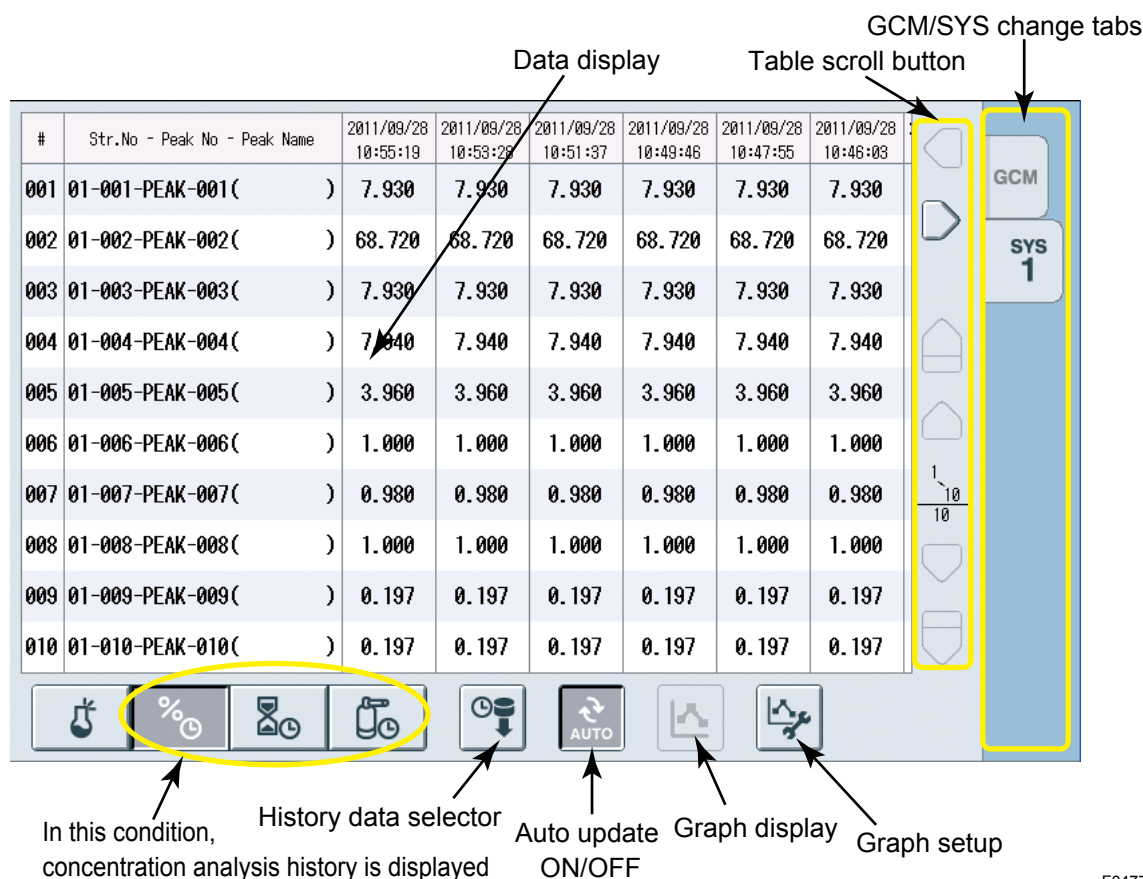
Figure 4.77 History Screen Layout
