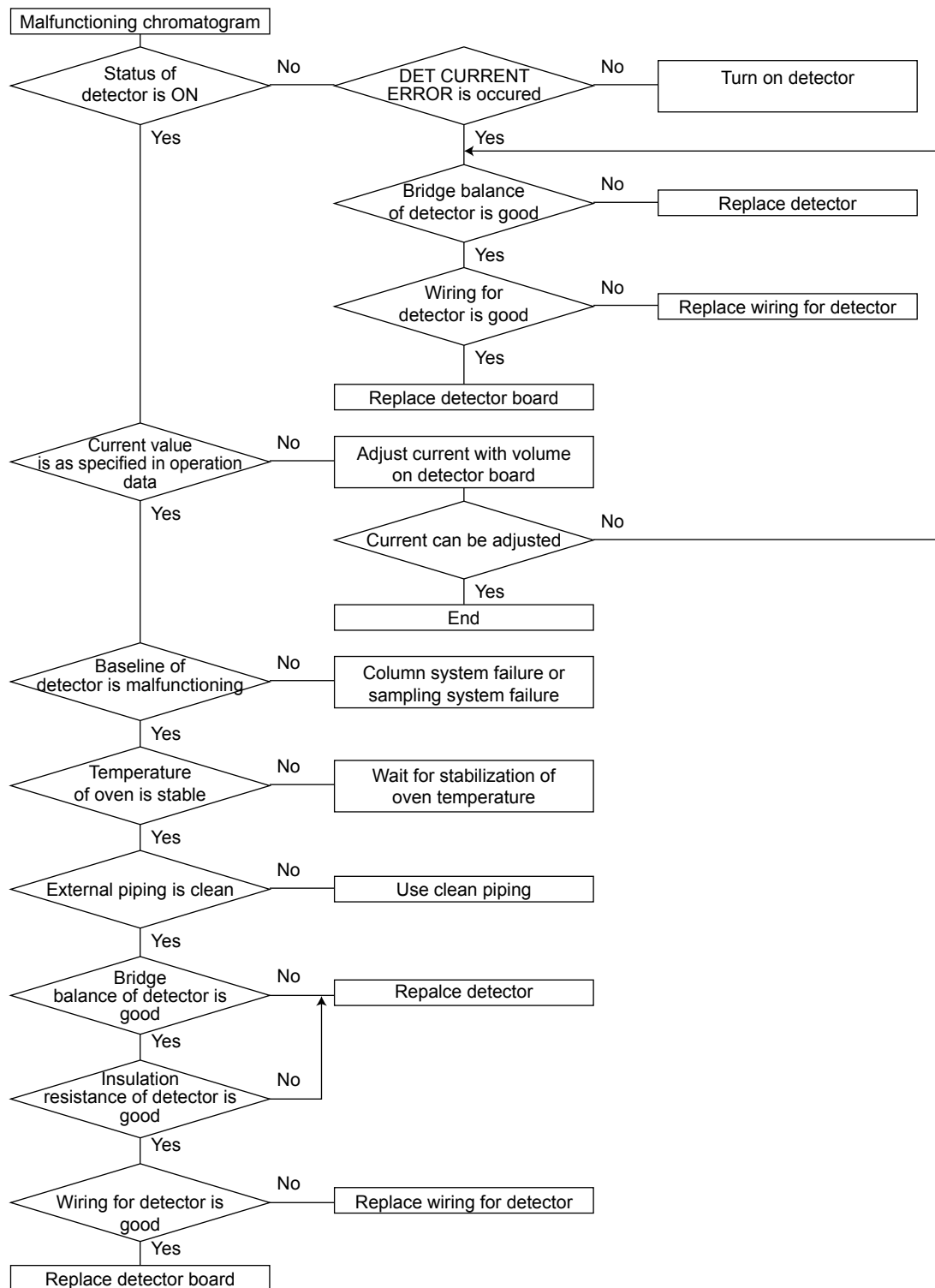
Figure 7.4 Troubleshooting Diagram for Malfunctioning Chromatogram (TCD)
