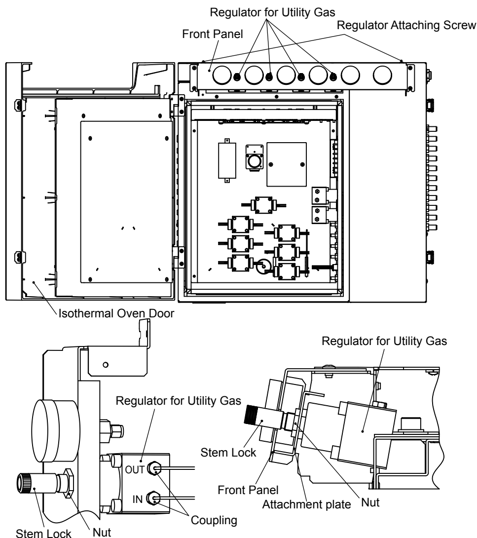
Figure 6.20 Regulator for Utility Gases
