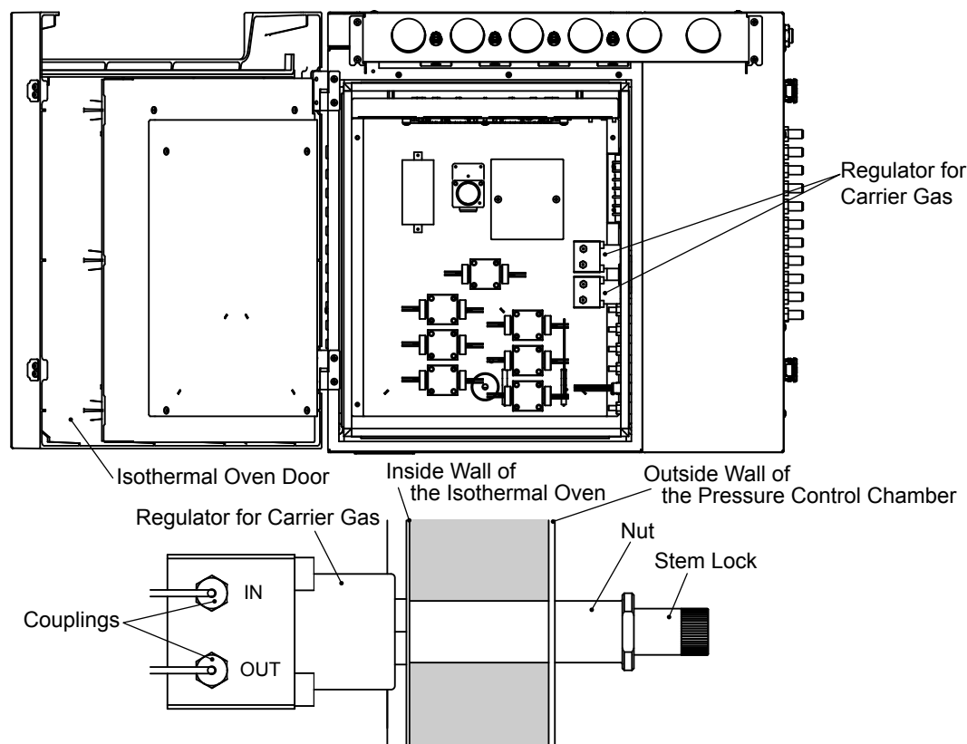
Figure 6.19 Regulator for carrier gas
