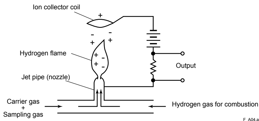
Figure 4 Fundamental Principle of Flame Ionization Detector
