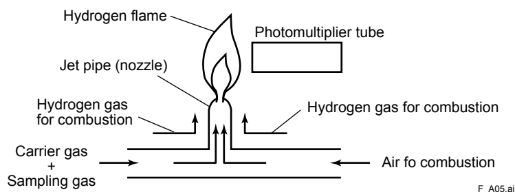
Figure 5 Basic Configuration of Flame Photometric Detector
