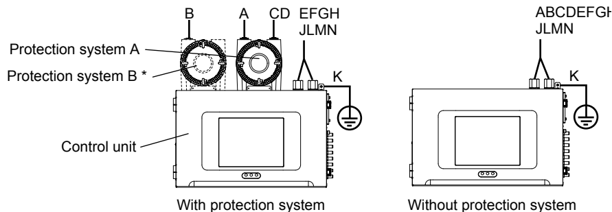
Figure 2.11 Cable connection locations
