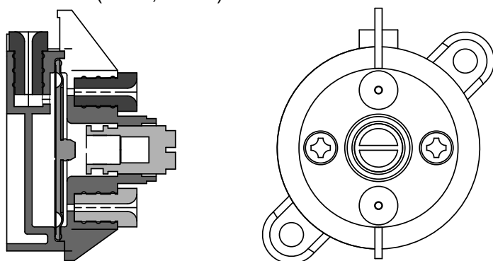
Figure 6.4 Pressure Switch for Detecting Internal Pressure
