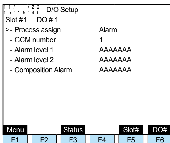
Figure 5.93 Example of D/O setup screen (setting the Process assign to Alarm)
