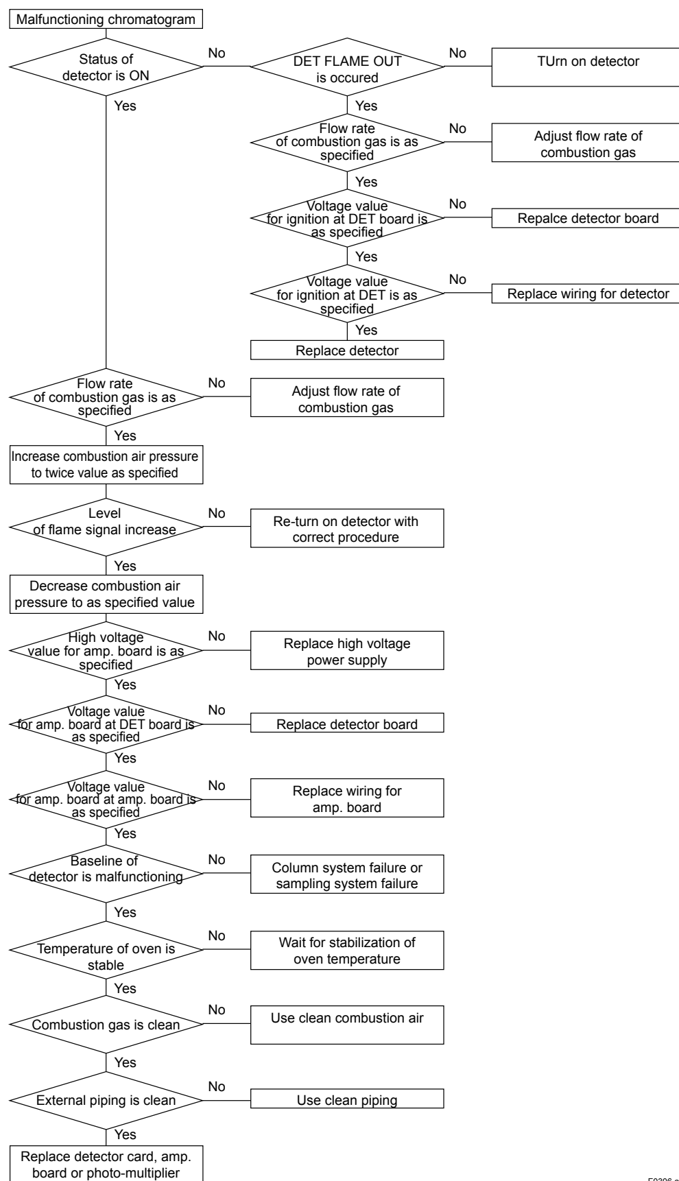
Figure 7.6 Troubleshooting Diagram for Malfunctioning Chromatogram (FPD)
