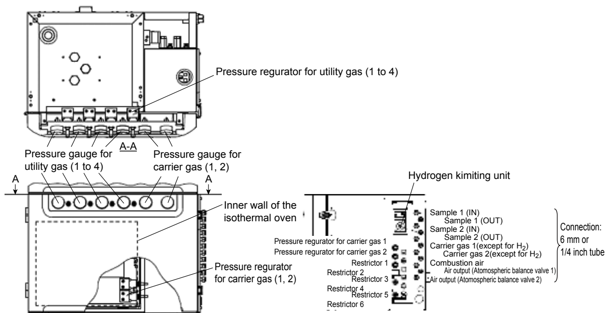
Figure 1.9 Pressure and flow control section of the isothermal oven
