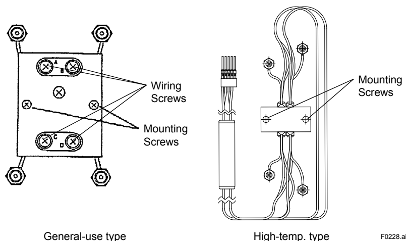
Figure 6.28 TCD
