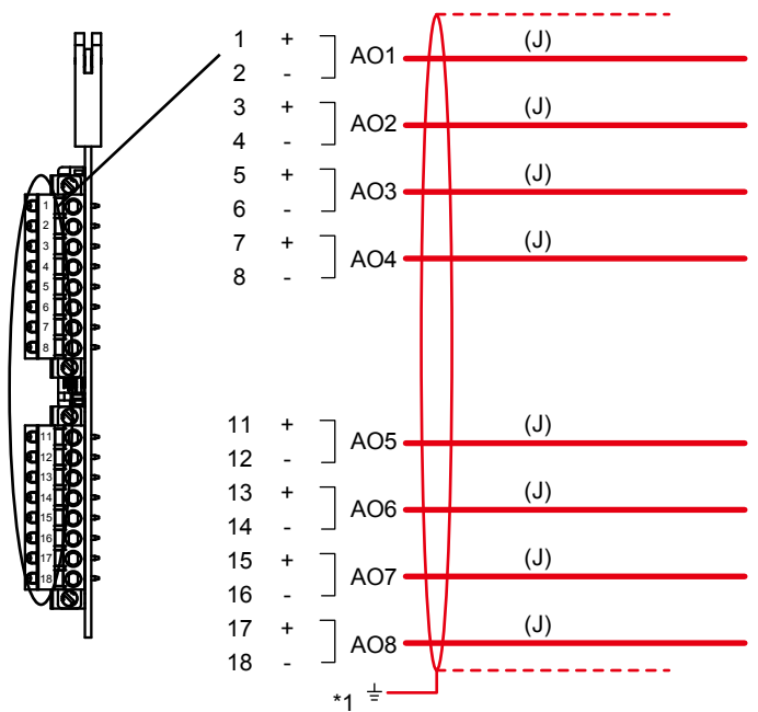
Figure 2.29 Wiring for an analog output card
