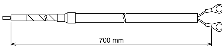
Figure 6.27 Temperature Sensor
