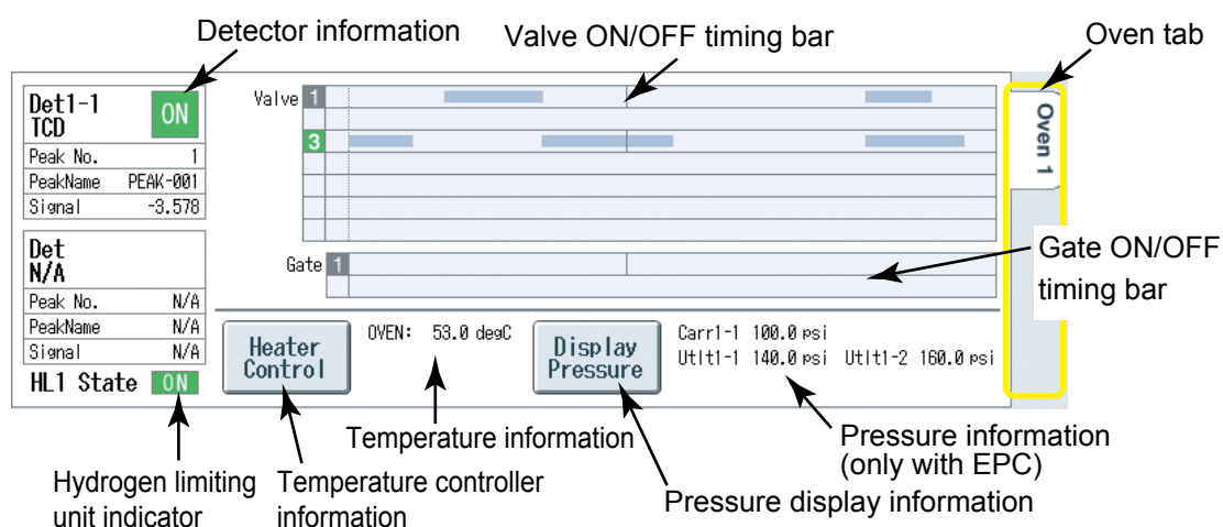
Figure 4.53 Example of Oven Information Display Area
