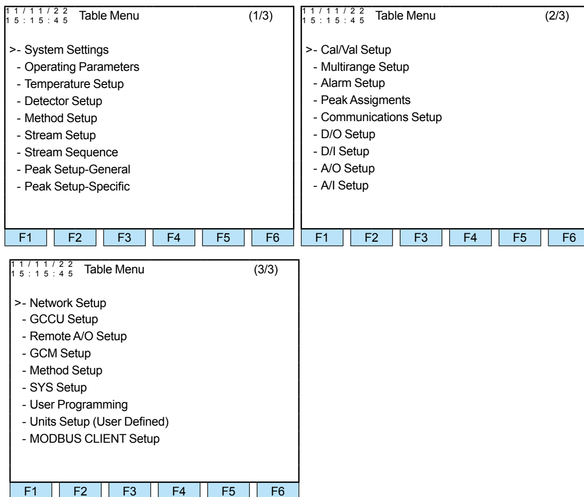
Figure 5.51 Table menu screen
