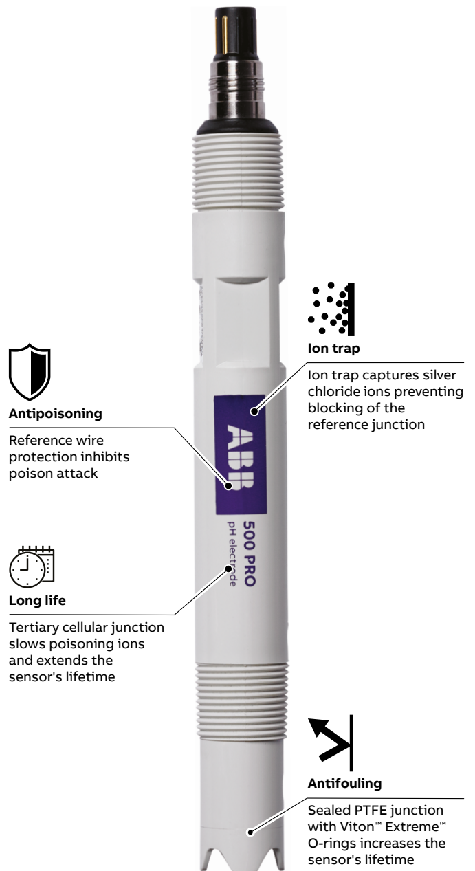
Figure 1 Sensor features
