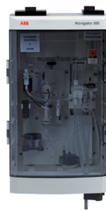
Hydrazine
