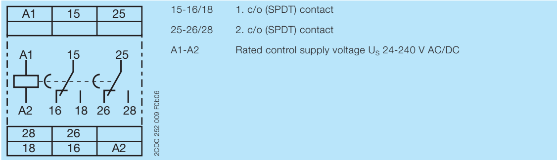
Connection diagram
