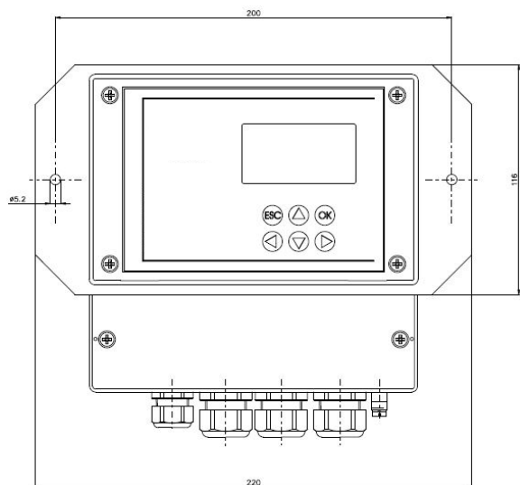
Panel mount model Panel cut out size: 166mm x 107mm
