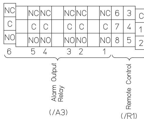
/A3/R1 Combination
