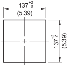
Single-unit Mounting
