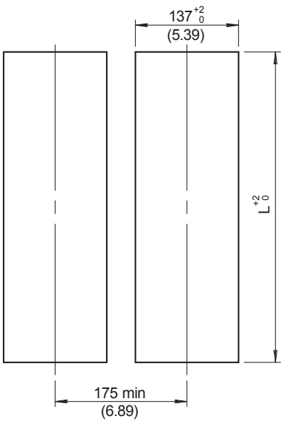
Side-by-side Mounting (vertically, max. 3 units)
