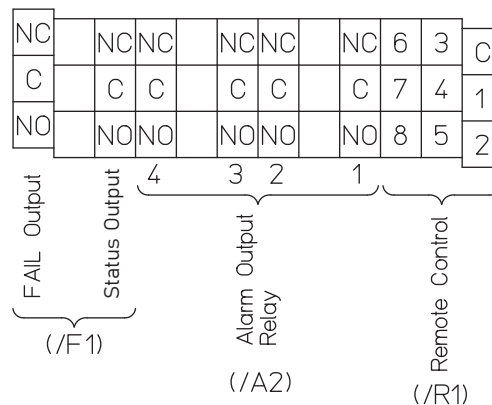
/A2/F1/R1 Combination
